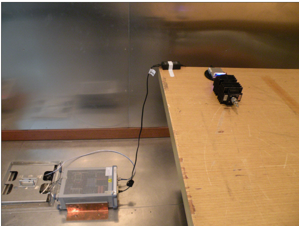
AC Line Conducted Emission Test Setup – Antenna Termination
