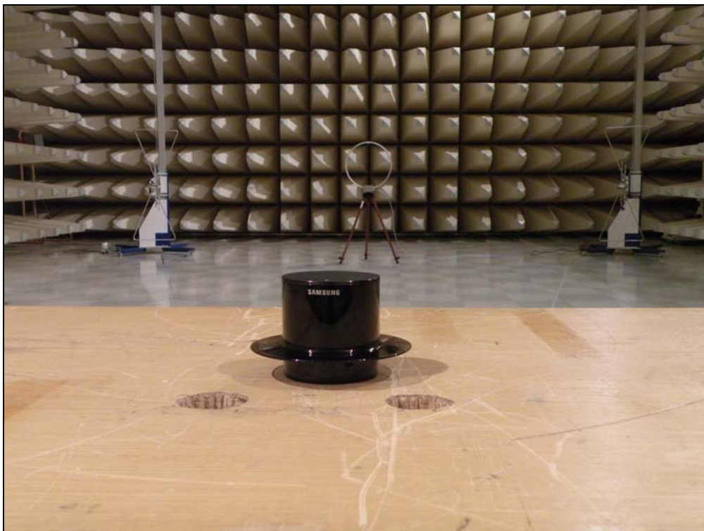
Loop Antenna Setup at 10m distance
