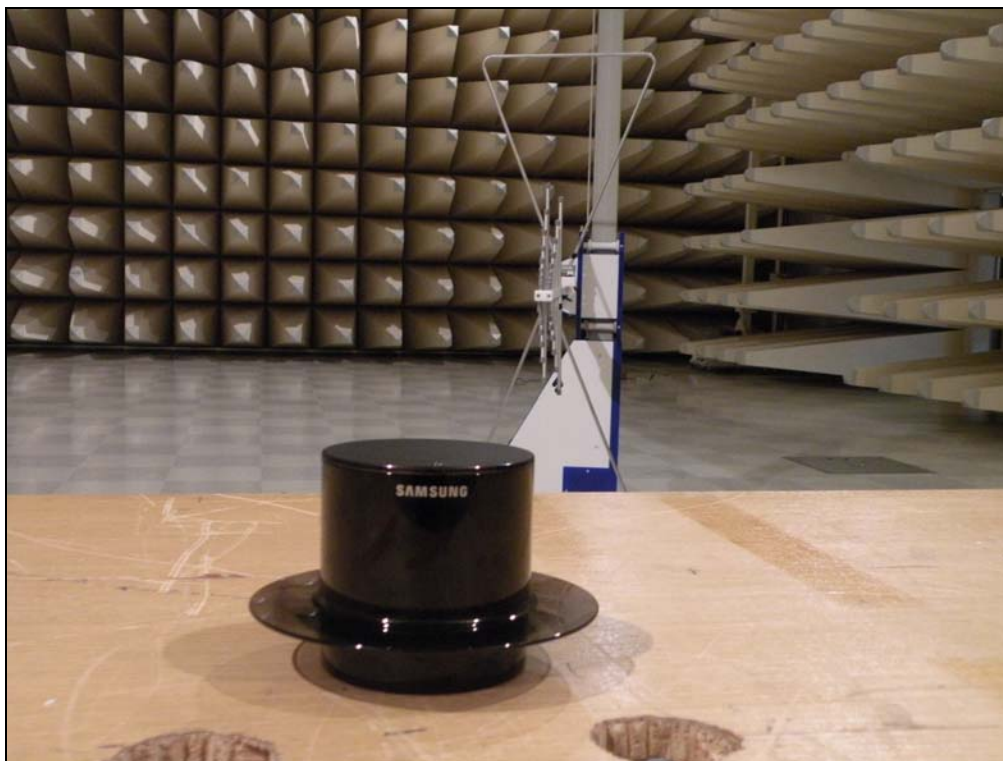
Biconi-Log Antenna Setup at 3m distance
