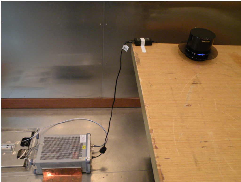
AC Line Conducted Emission Test Setup- Normal Operation
