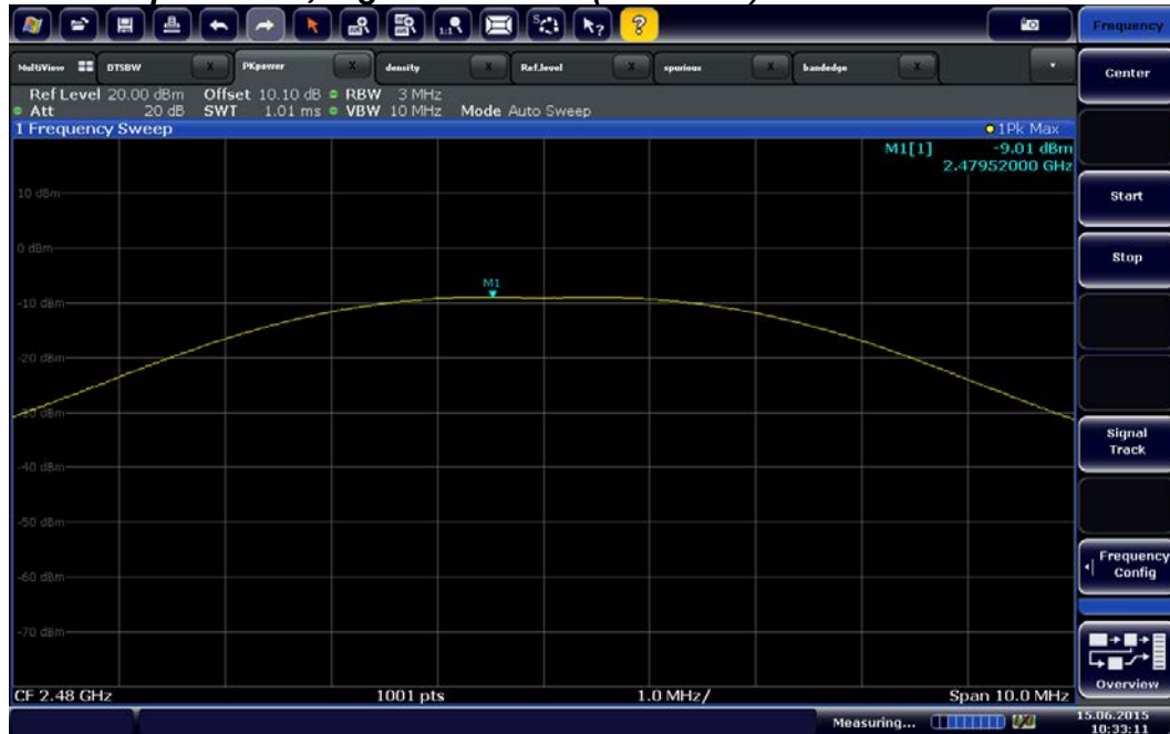
Peak Output Power, Highest Channel (2480 MHz)
