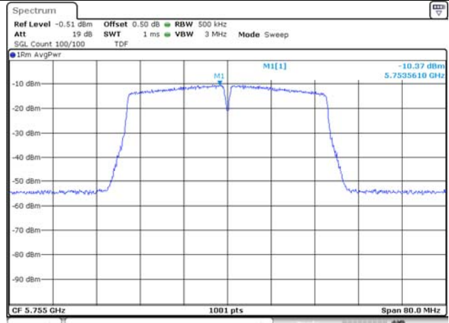
UNII-3 / 802.11ac VHT40 / Low ch.
