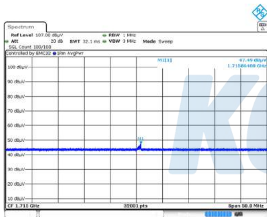
Average data (1 715.86 MHz)
