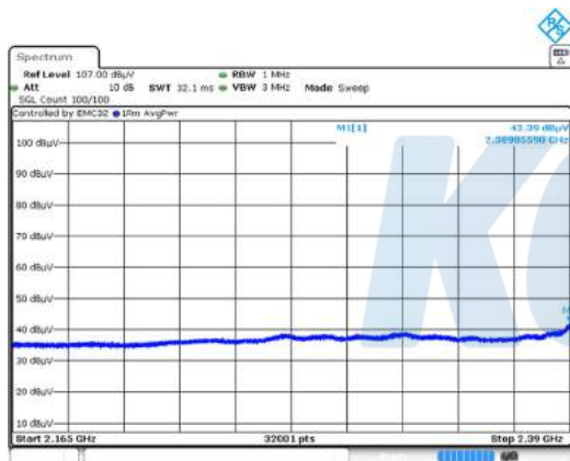
Average data (2 389.86 MHz)
