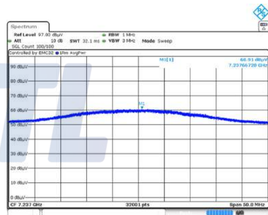
Average data (7 237.67 MHz)
