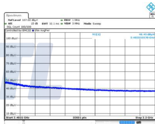
Average data (2 483.51 MHz)
