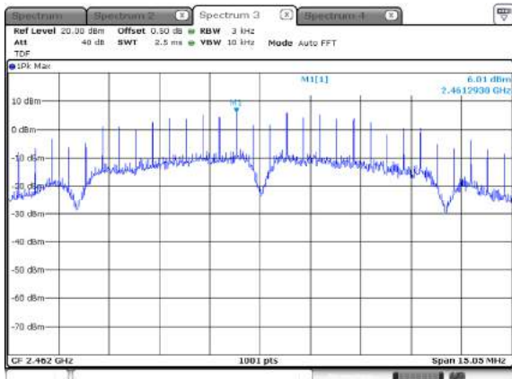
802.11b / High ch.
