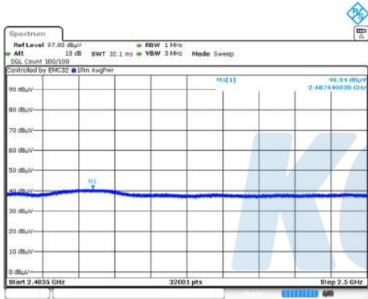
Average data (2 486.70 MHz)
