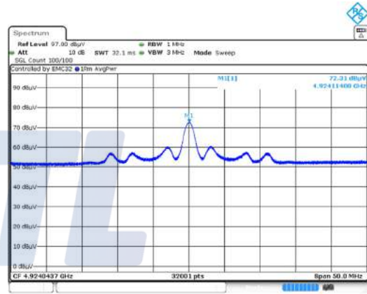
Average data (4 924.11 MHz)
