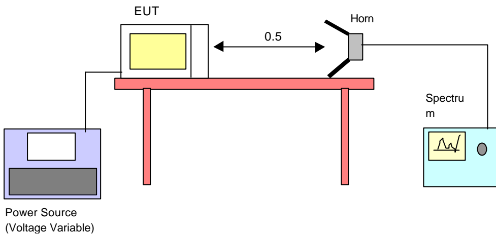
Fig. 4 Operating Frequency Measurements Configuration
