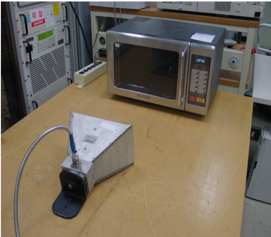
Fig. 5 Test Setup for Operating Frequency Measurements
