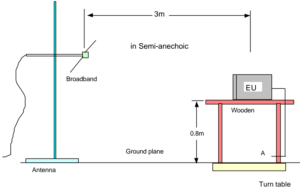
Fig. 6 Radiated Emission Configuration(30 - 1000MHz)
