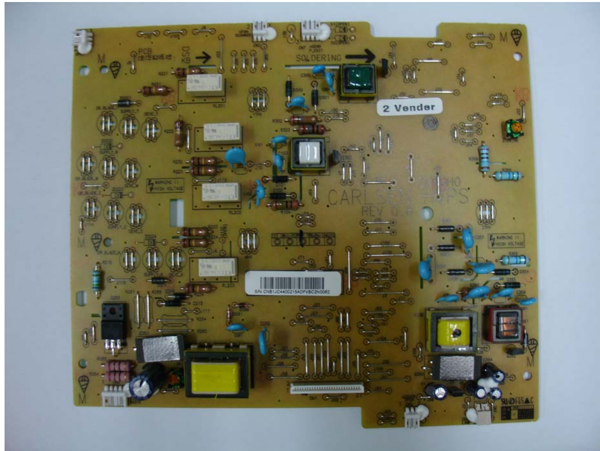
PBA Photo_HVPS PBA_Top
