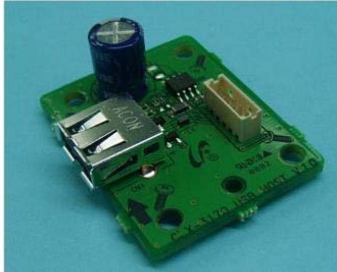
PBA Photo_USB Host PBA_Top
