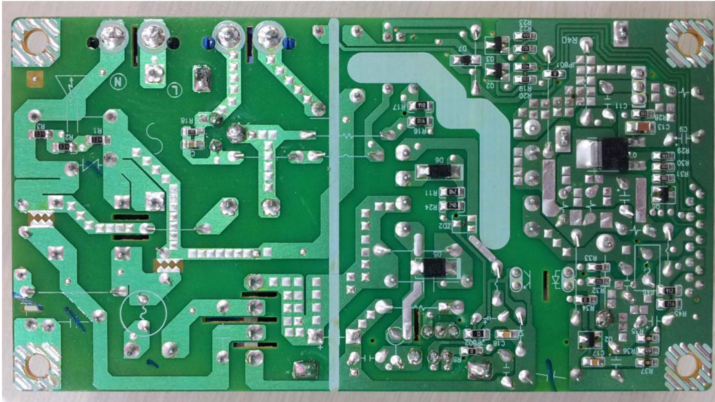
PBA Photo_SMPS PBA_Bottom
