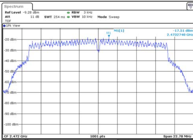
802.11g / 2 472 MHz
