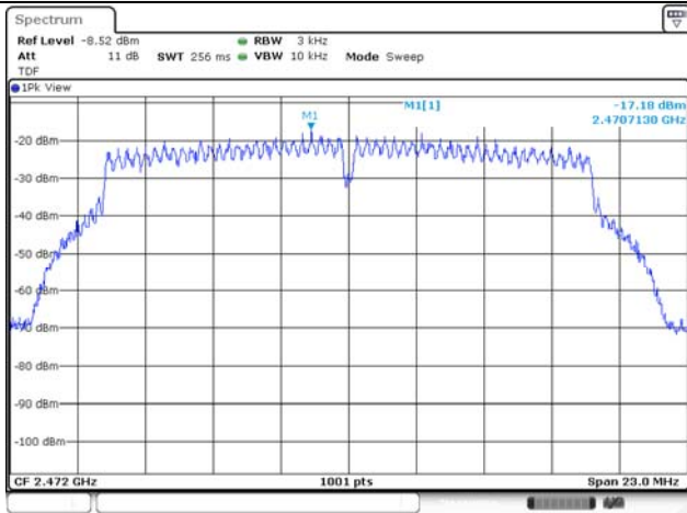
802.11g / 2 472 MHz
