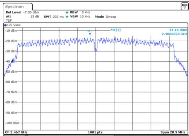
802.11n HT20 / 2 467 MHz
