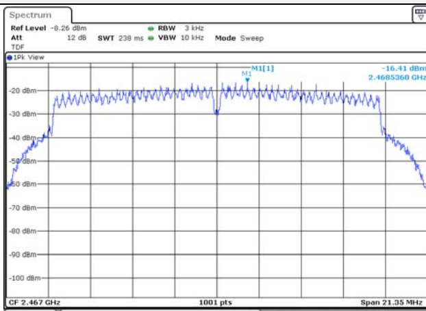
802.11g / 2 467 MHz
