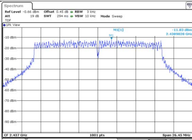
802.11n HT20 / 2 437 MHz
