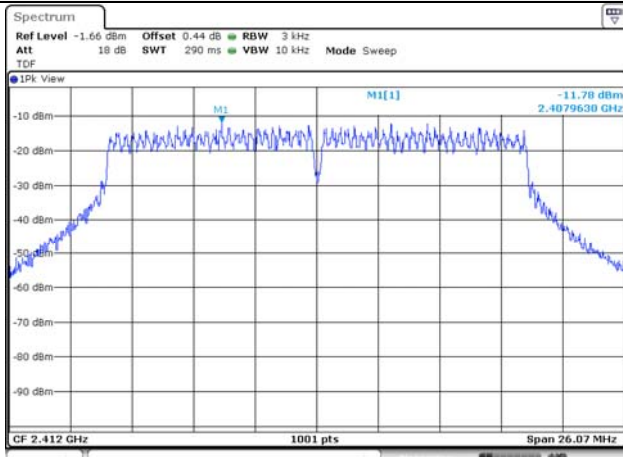
802.11n HT20 / 2 412 MHz
