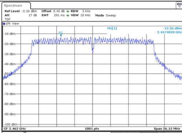
802.11n HT20 / 2 462 MHz
