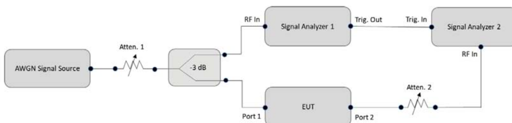
Figure 2. Contention-based protocol test setup, conducted method
