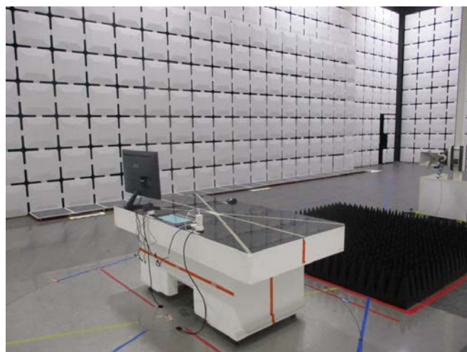
REAR VIEW #2(18 ~ 26.5 GHZ)
