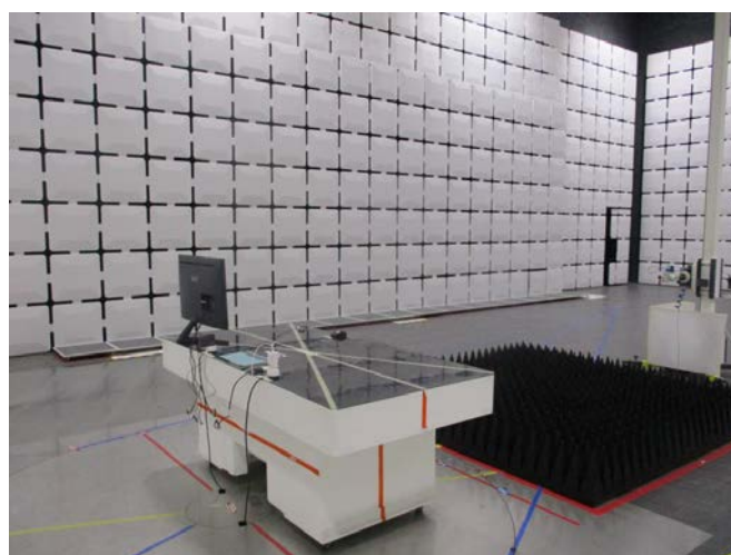
REAR VIEW #2 (26.5 ~40 GHZ)
