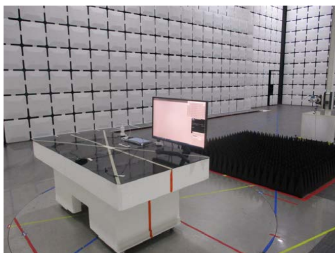
FRONT VIEW #2 (26.5 ~ 40 GHZ)
