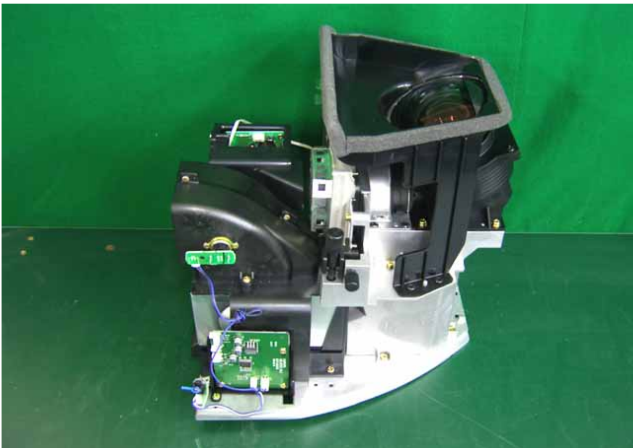
Engine ass'y- 1 view
