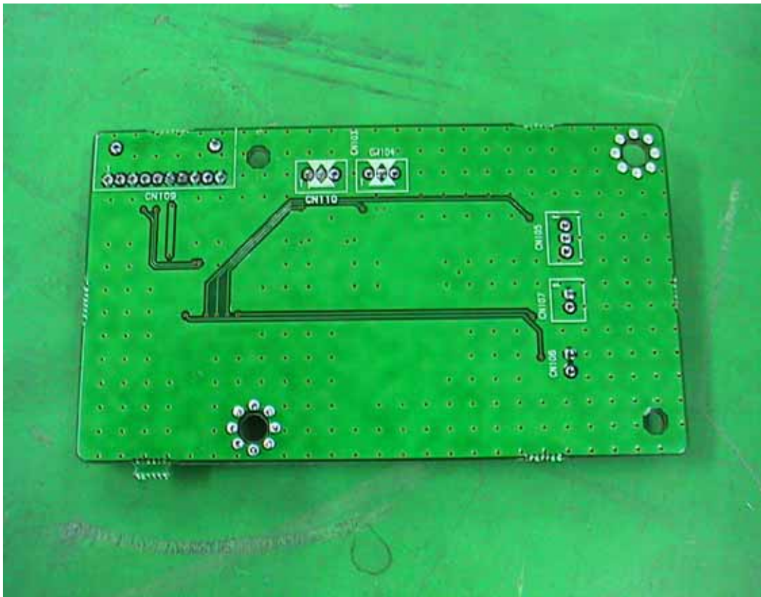
Sub detect board top view
