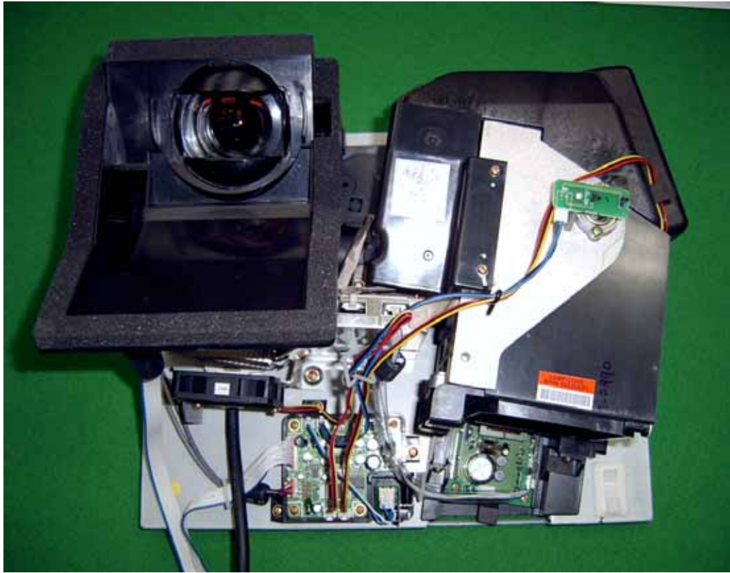
Engine view
