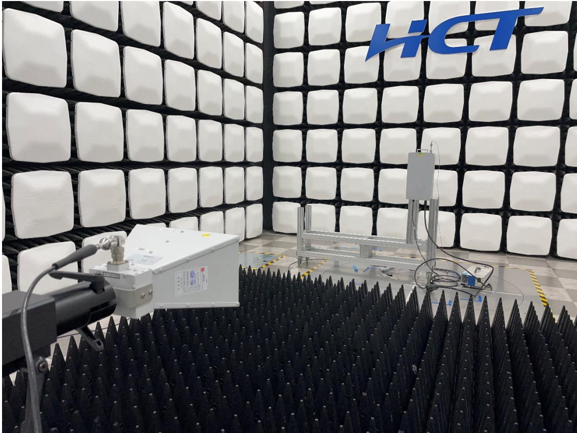
Radiated Test Setup Photo –Spurious (9120D Horn Antenna, Vertical)
