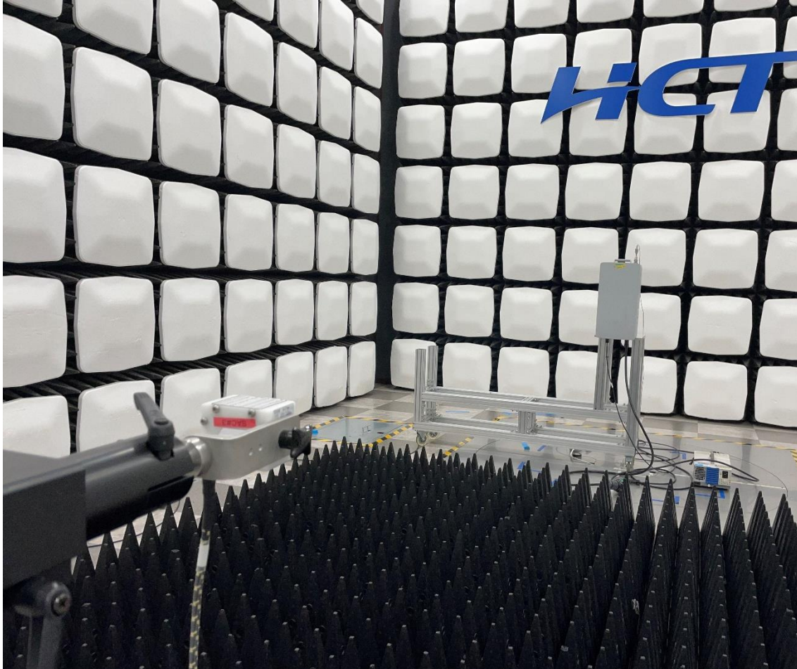
Radiated Test Setup Photo – Spurious (9170 Horn Antenna, Horizontal)
