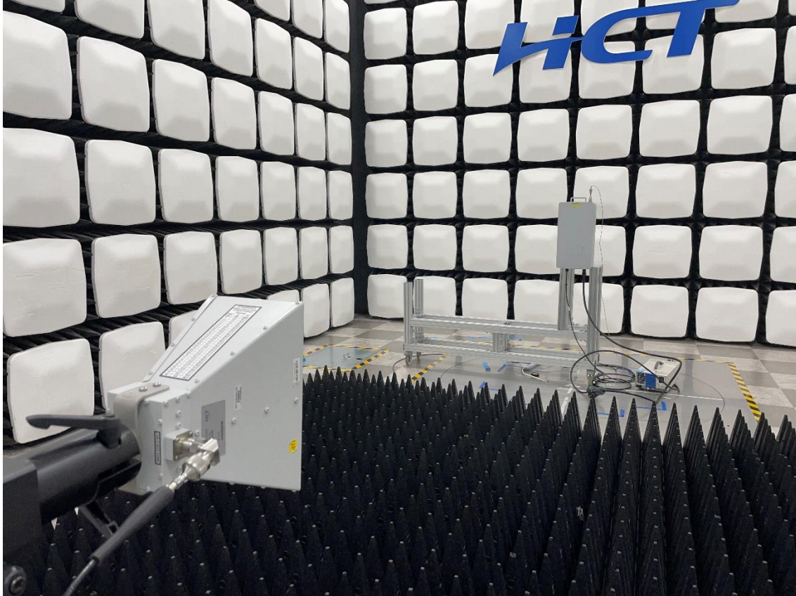
Radiated Test Setup Photo – Spurious (9120D Horn Antenna, Horizontal)
