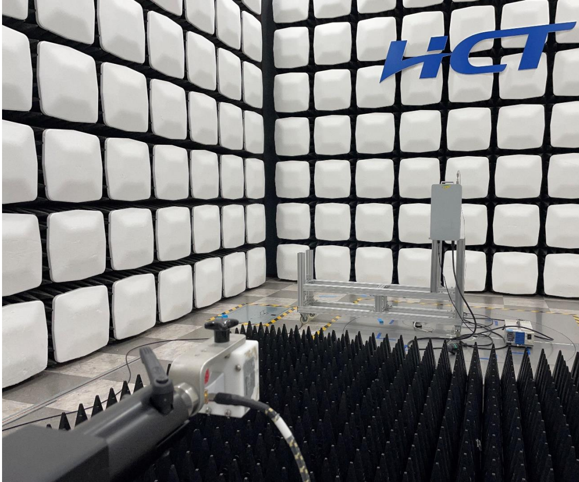
Radiated Test Setup Photo –Spurious (9170 Horn Antenna, Vertical)
