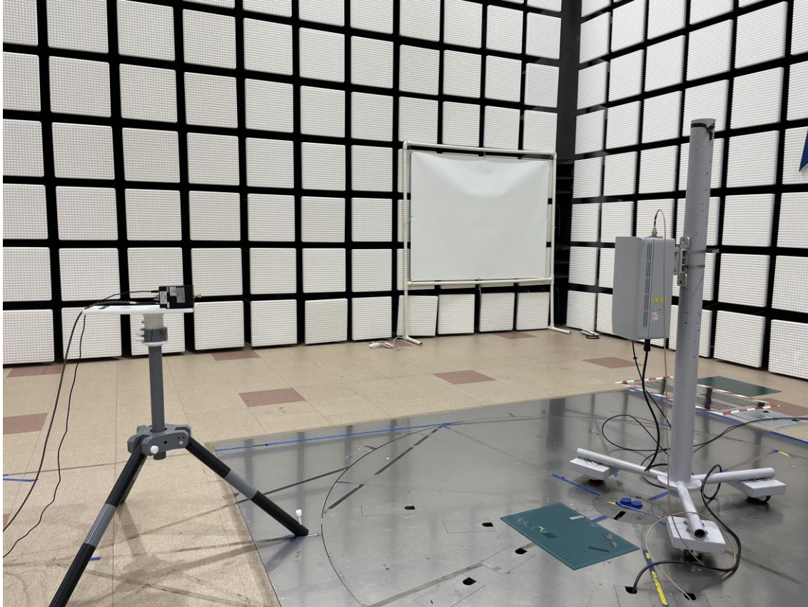
Radiated Test Setup Photo – Spurious (WR-05 Horn Antenna, Horizontal)
