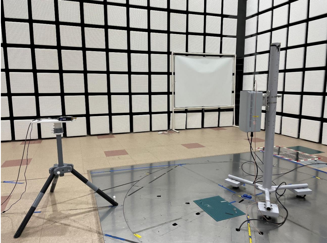
Radiated Test Setup Photo – Spurious (WR-08 Horn Antenna, Vertical)
