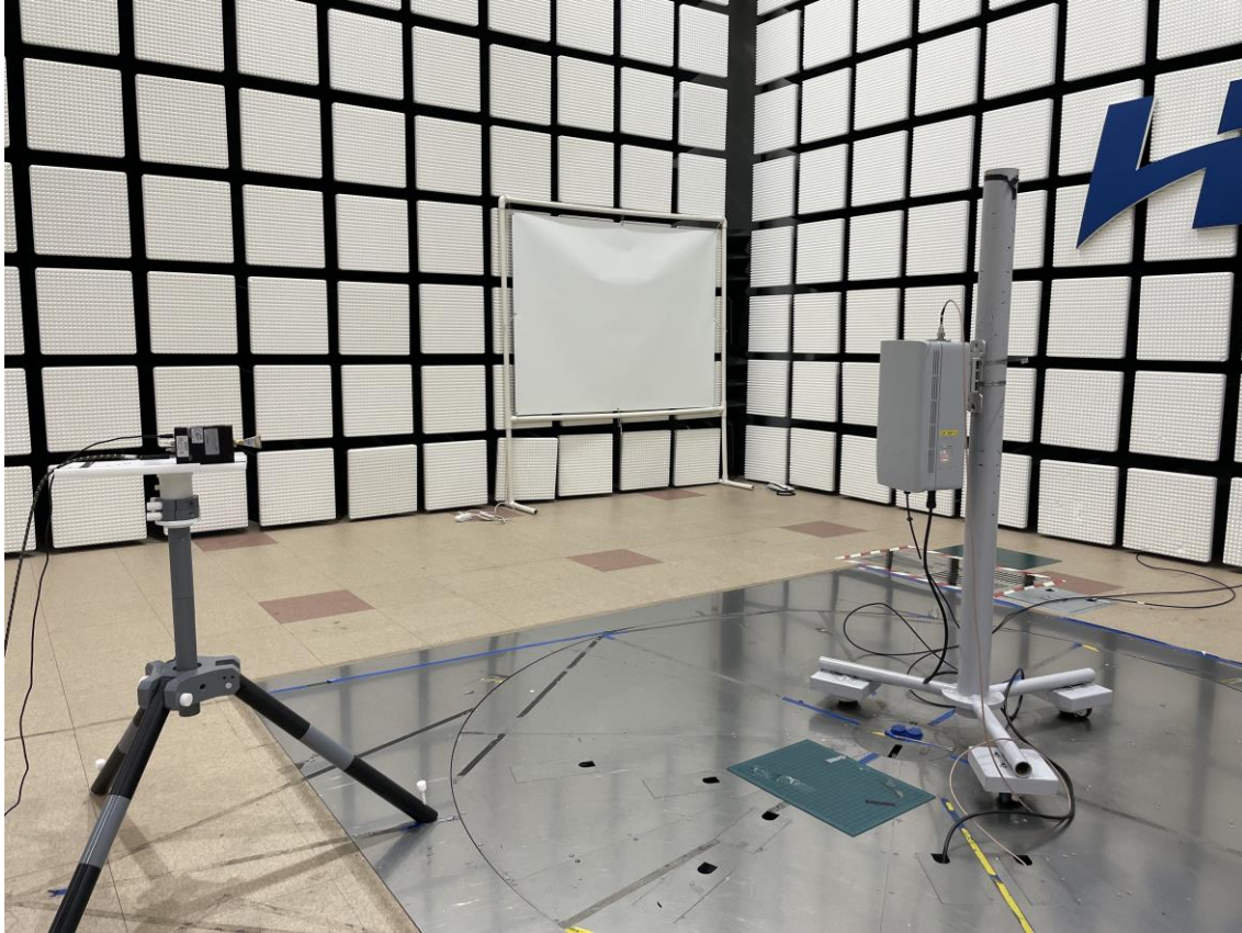
Radiated Test Setup Photo – Spurious (WR-12 Horn Antenna, Horizontal)
