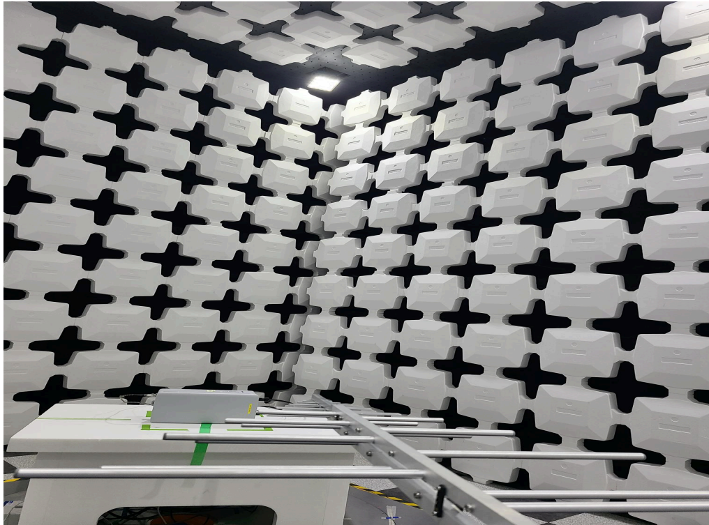
Testing setup for 30 MHz to 1 GHz
