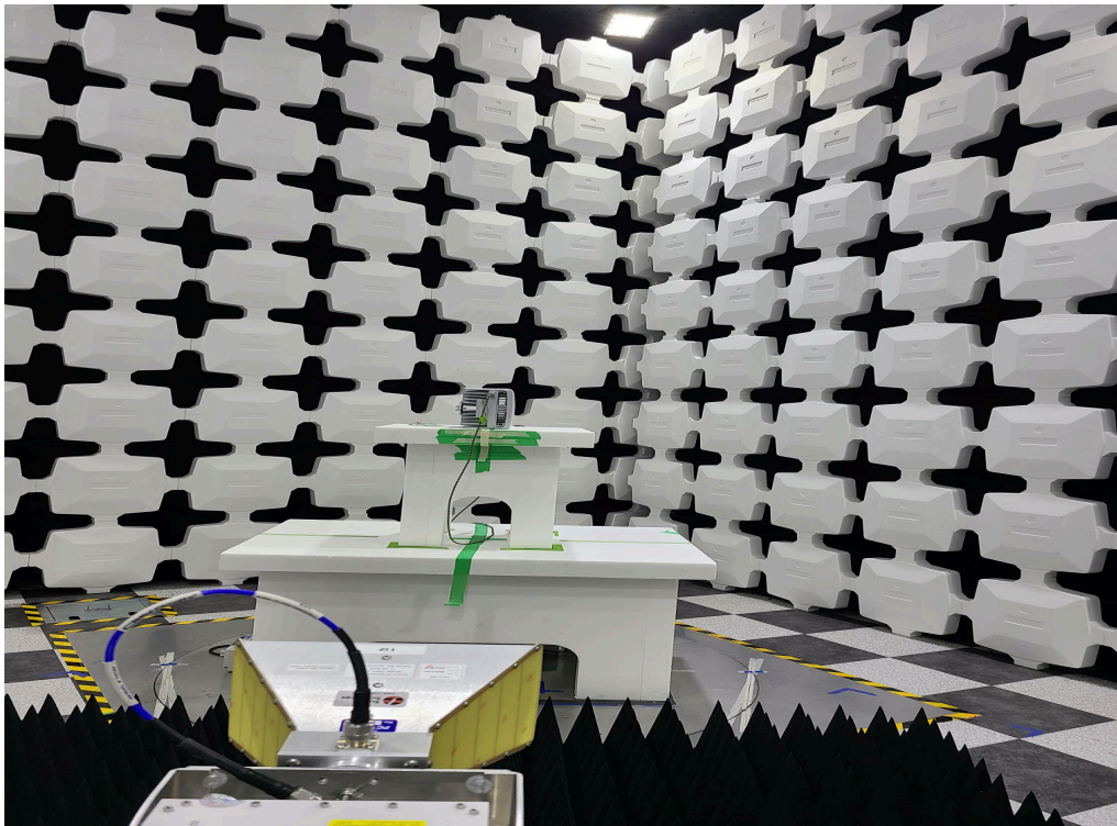
Testing setup for 1 GHz to 18 GHz
