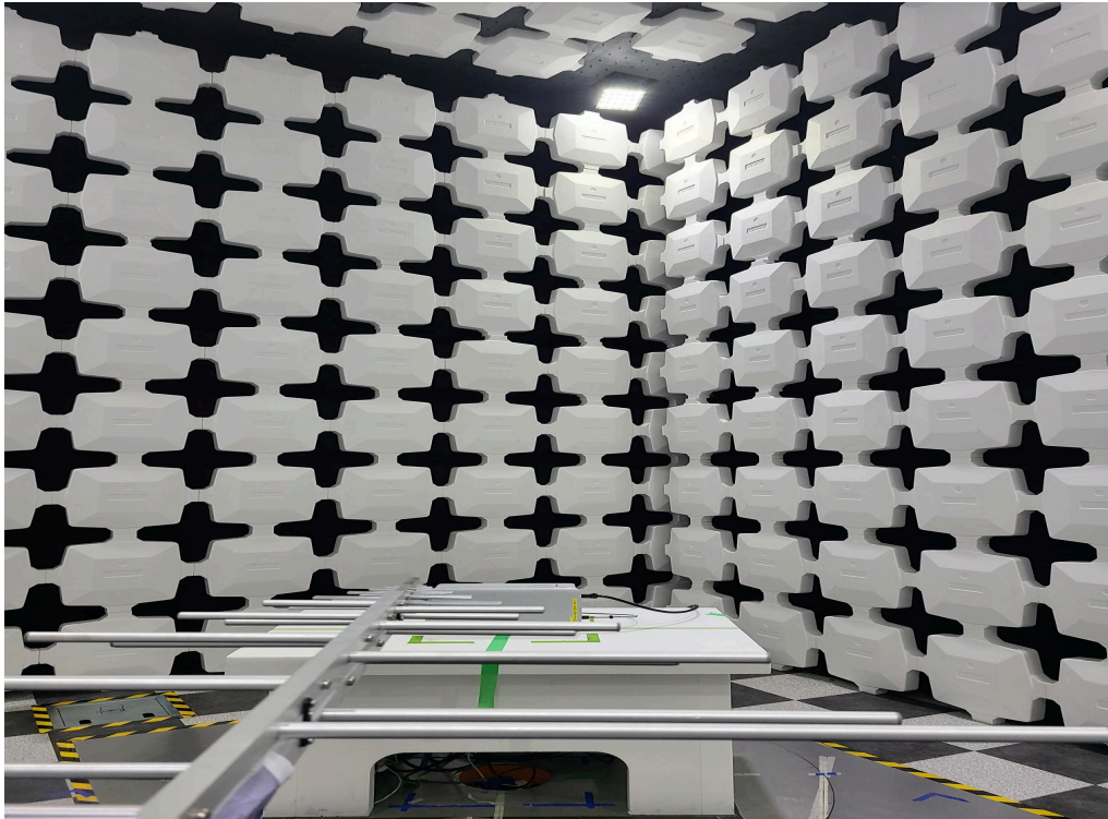
Testing setup for 30 MHz to 1 GHz
