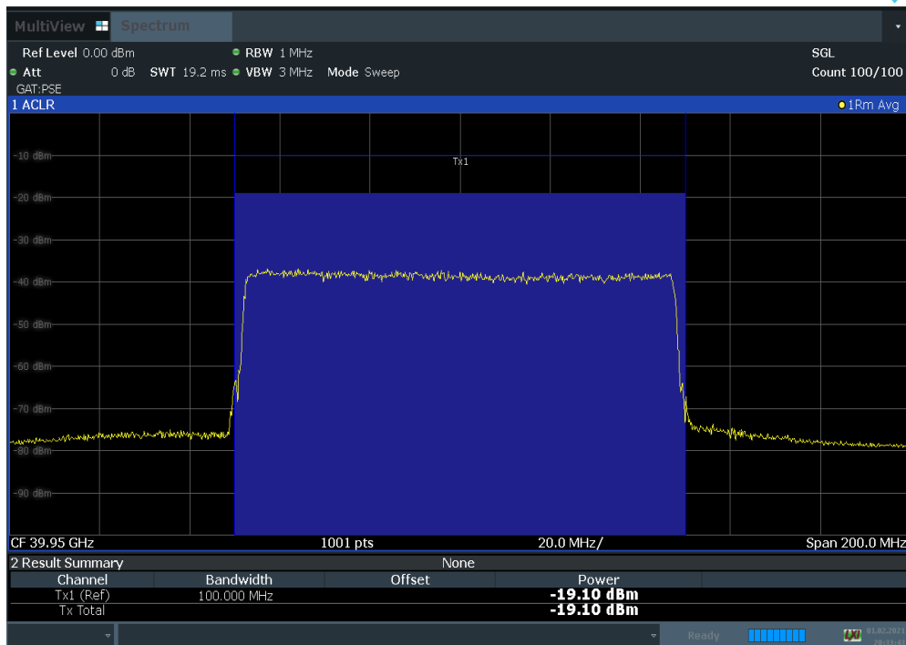
Plot 7-44. Antenna A EIRP Density Plot (100 MHz BW 1CC 16QAM High Channel)
