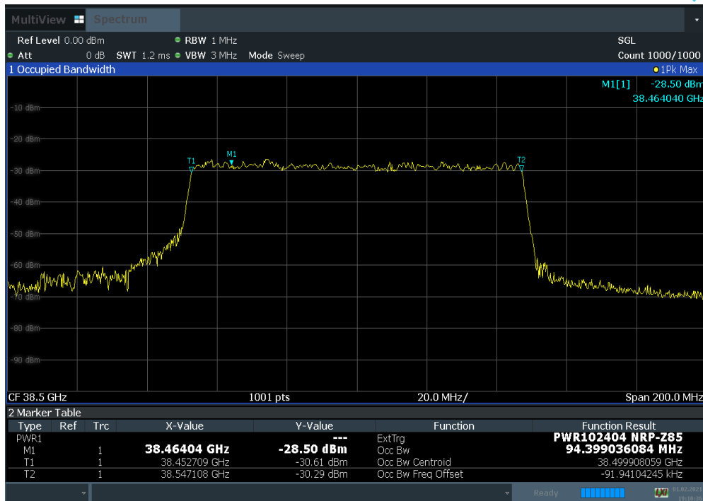
Plot 7-14. Occupied Bandwidth Plot (100 MHz 1CC BW 16QAM Mid Channel)
