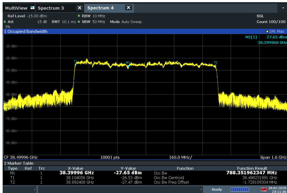
Plot 7-23. Occupied Bandwidth Plot (100MHz BW 8CC 16QAM Mid Channel)
