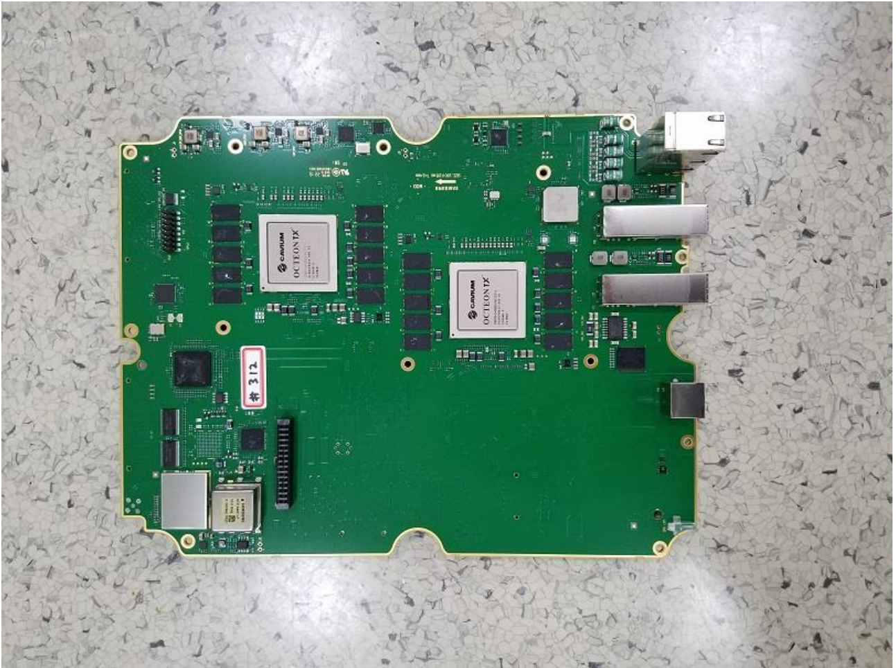
[G7DA Module_Bottom]
