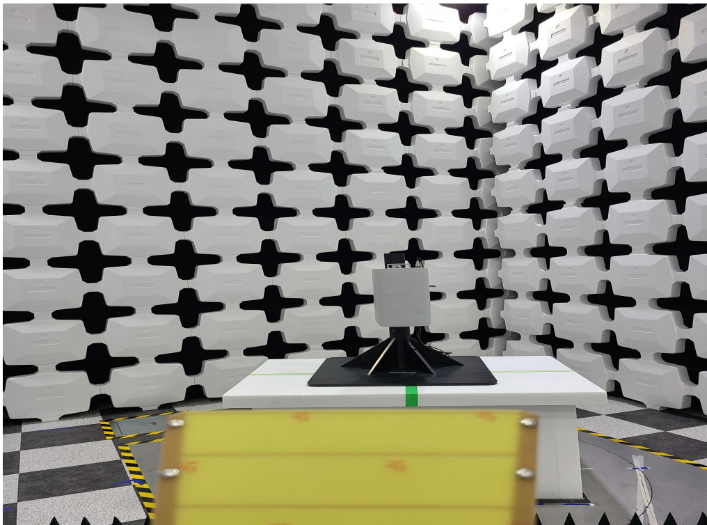
Testing setup for 1 GHz to 18 GHz
