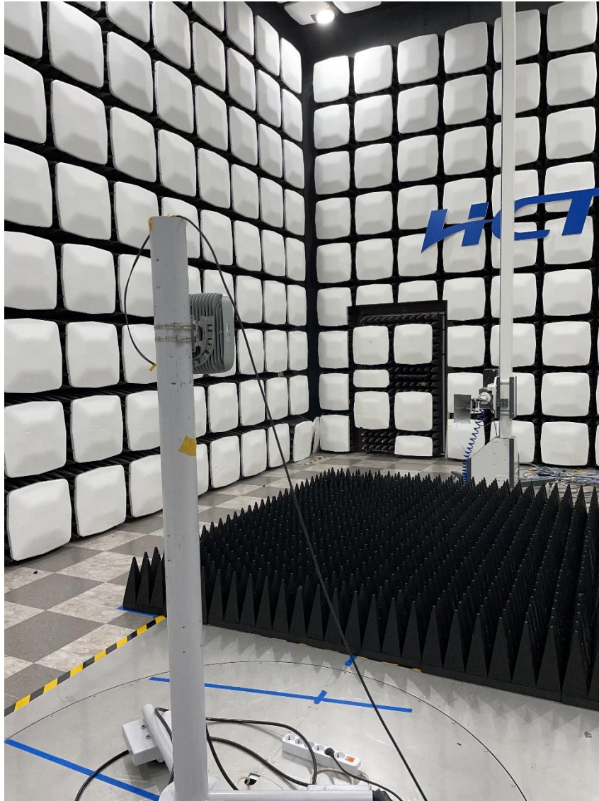
Radiated Test Setup Photo – Spurious (Horn Antenna 1 M, Horizontal)
