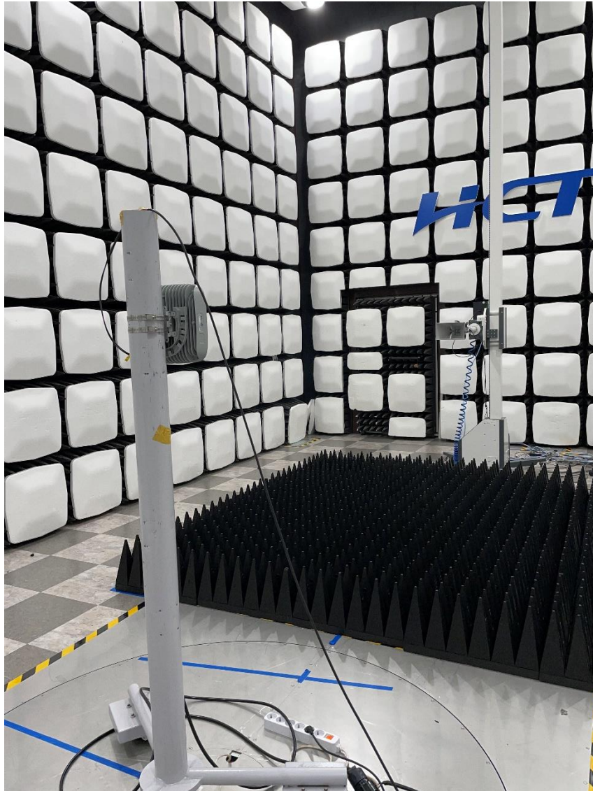
Radiated Test Setup Photo –Spurious (Horn Antenna 1.5 M, Vertical)
