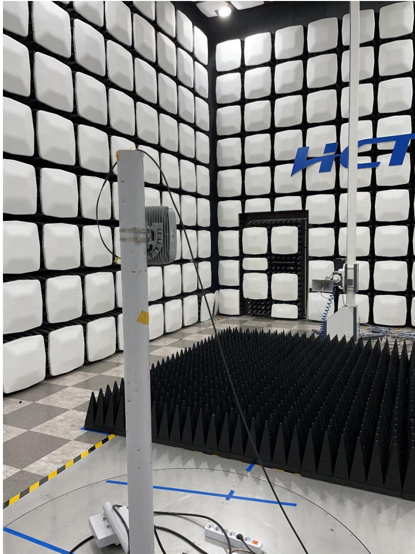
Radiated Test Setup Photo –Spurious (Horn Antenna 1 M, Vertical)
