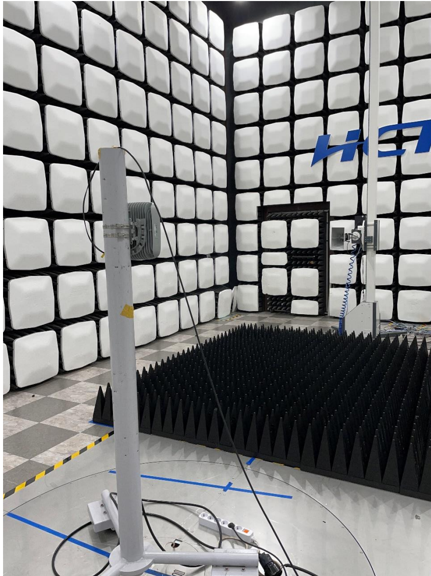
Radiated Test Setup Photo – Spurious (Horn Antenna 1.5 M, Horizontal)
