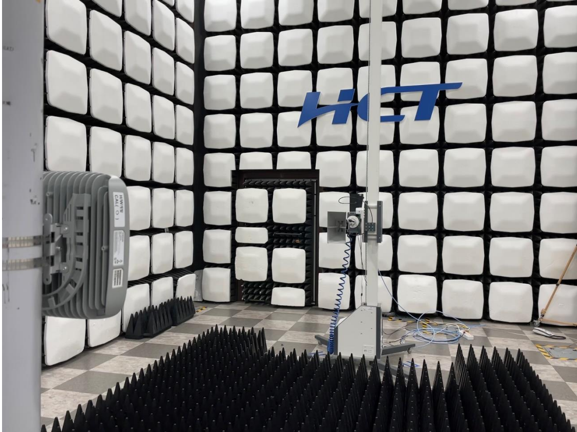
Radiated Test Setup Photo – Spurious (Horn Antenna, Horizontal)
