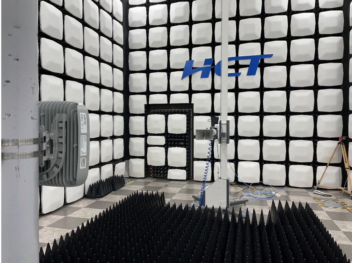
Radiated Test Setup Photo – Spurious (Horn Antenna, Vertical)
