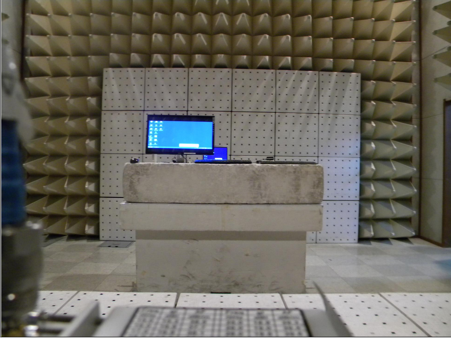
Radiated Emission (Above 1 GHz : 18 GHz~26 GHz) _ Front
