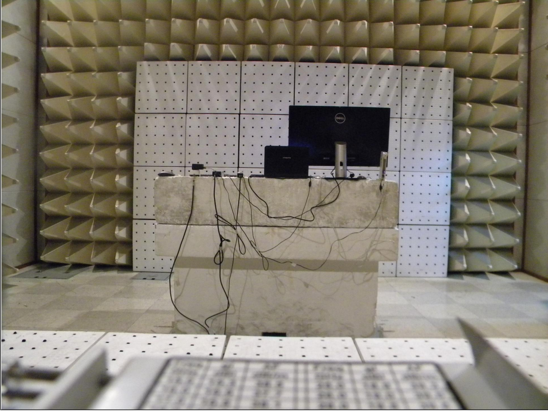
Radiated Emission (Above 1 GHz : 18 GHz~26 GHz) _ Rear
