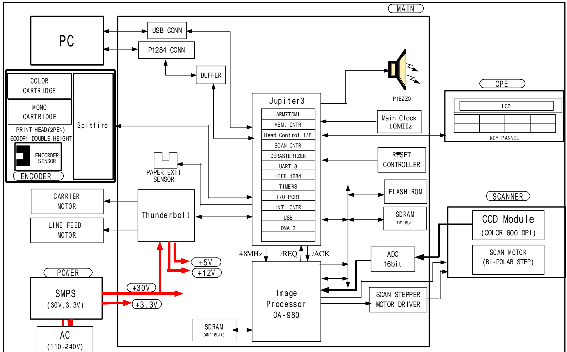
Block Diagram of A3000 Electrical Function
