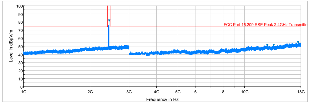
Plot 6-45. Radiated Spurious Plot above 1GHz (BT – Ch. 39, Ant. Pol. V)
