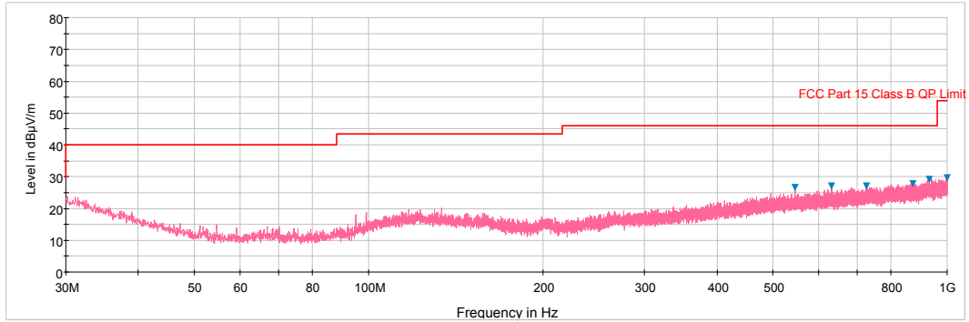
Plot 6-52. Radiated Spurious Plot below 1GHz (Pol. H)
