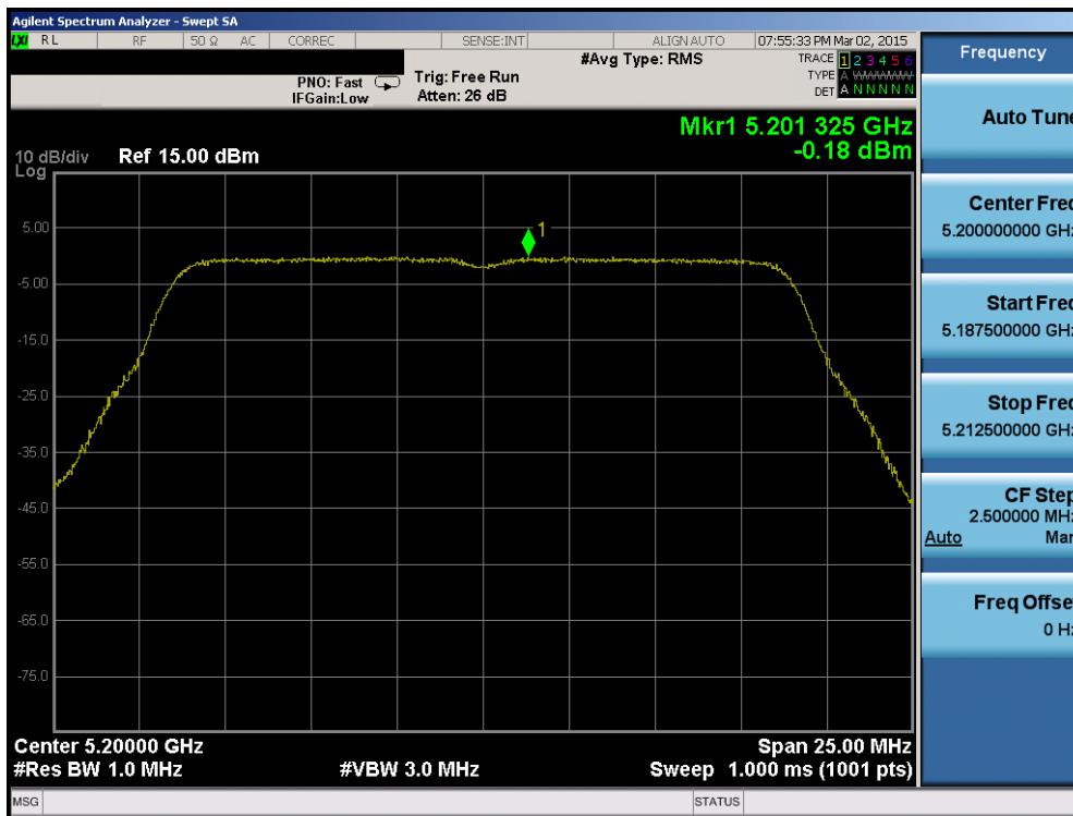
Plot 6-119. Power Spectral Density Plot (20MHz BW 802.11n (UNII Band 1) – Ch. 40)
