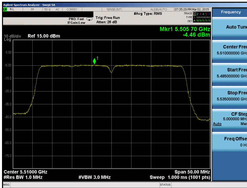
Plot 6-101. Power Spectral Density Plot (40MHz BW 802.11n (UNII Band 2C) – Ch. 102)
