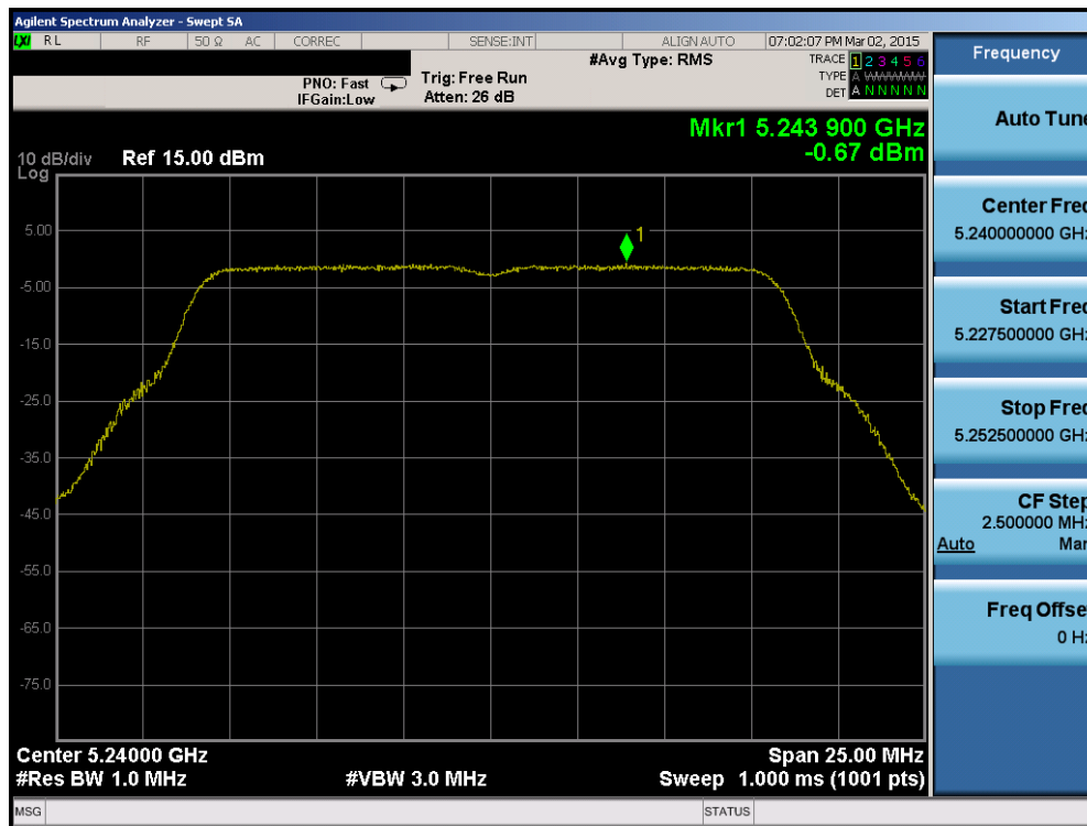
Plot 6-79. Power Spectral Density Plot (802.11a (UNII Band 1) – Ch. 48)
