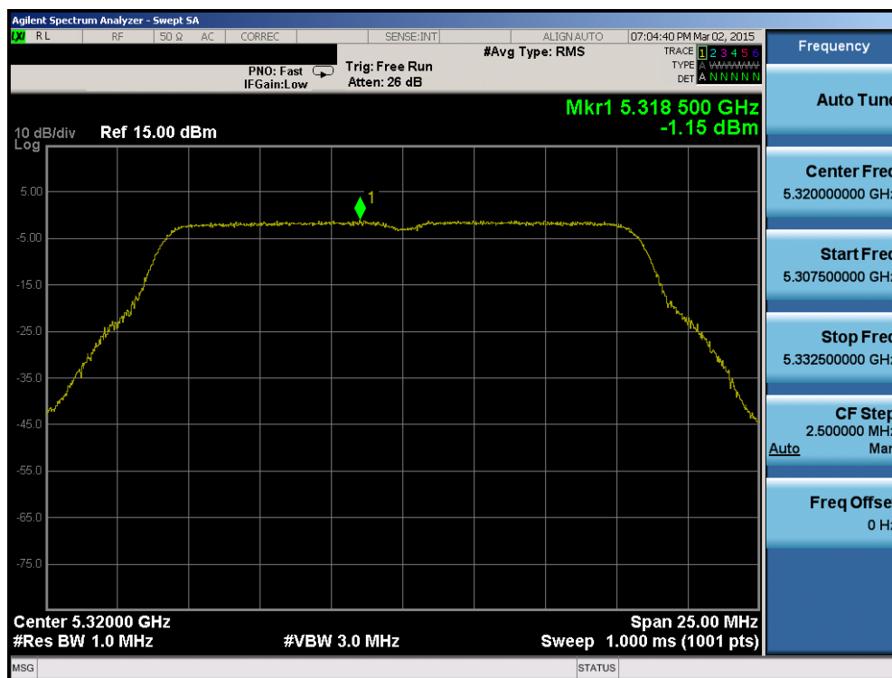
Plot 6-88. Power Spectral Density Plot (802.11a (UNII Band 2A) – Ch. 64)
