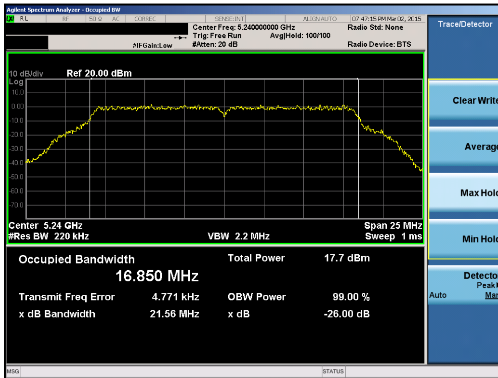
Plot 6-32. 26dB Bandwidth Plot (802.11a (UNII Band 1) – Ch. 48)
