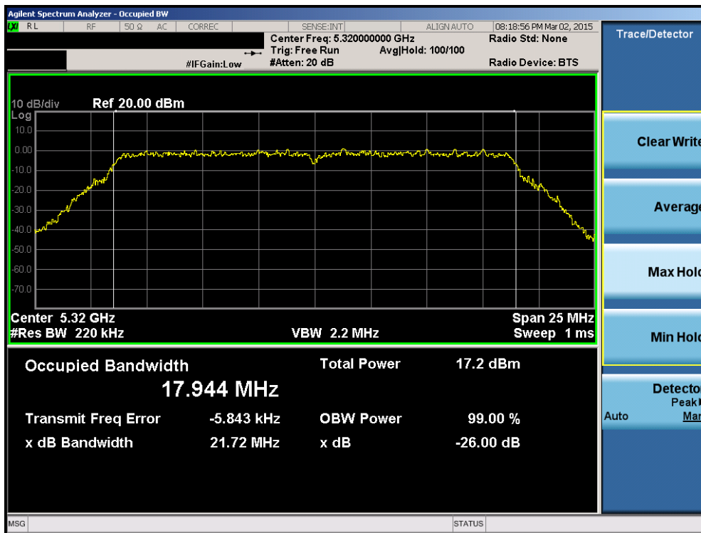
Plot 6-44. 26dB Bandwidth Plot (20MHz BW 802.11n (UNII Band 2A) – Ch. 64)
