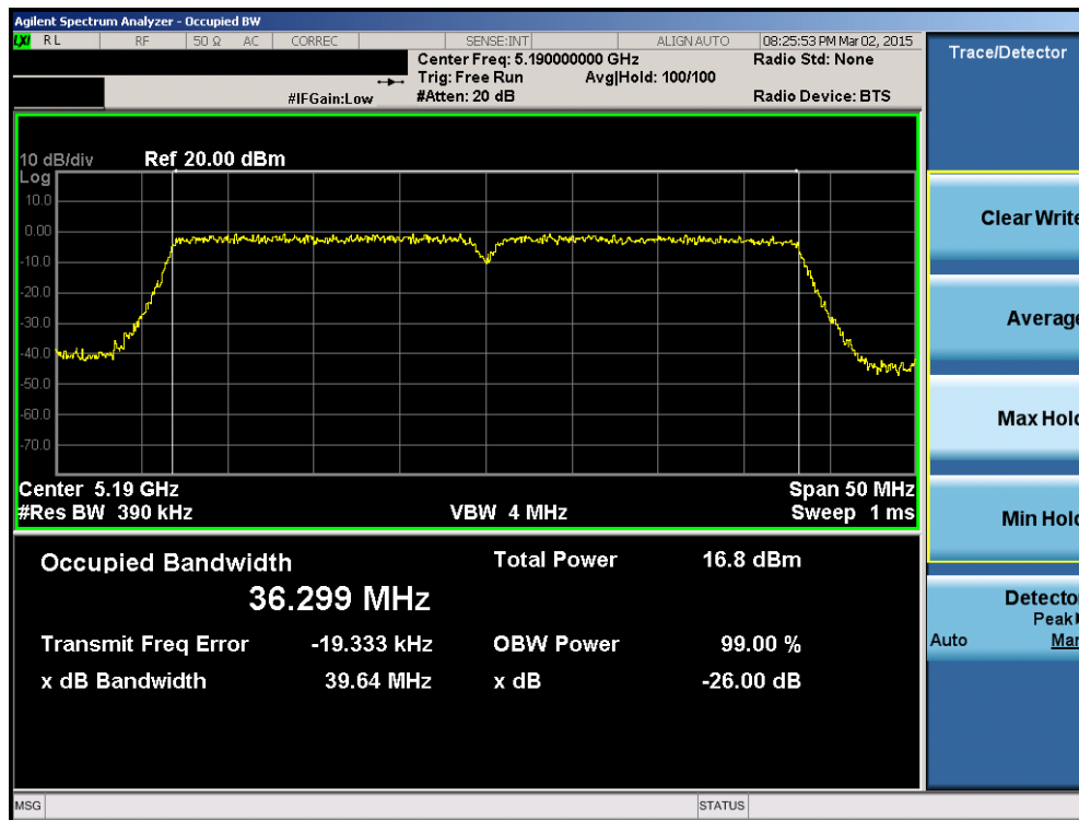
Plot 6-36. 26dB Bandwidth Plot (40MHz BW 802.11n (UNII Band 1) – Ch. 38)
