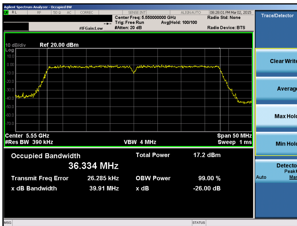
Plot 6-55. 26dB Bandwidth Plot (40MHz BW 802.11n (UNII Band 2C) – Ch. 110)
