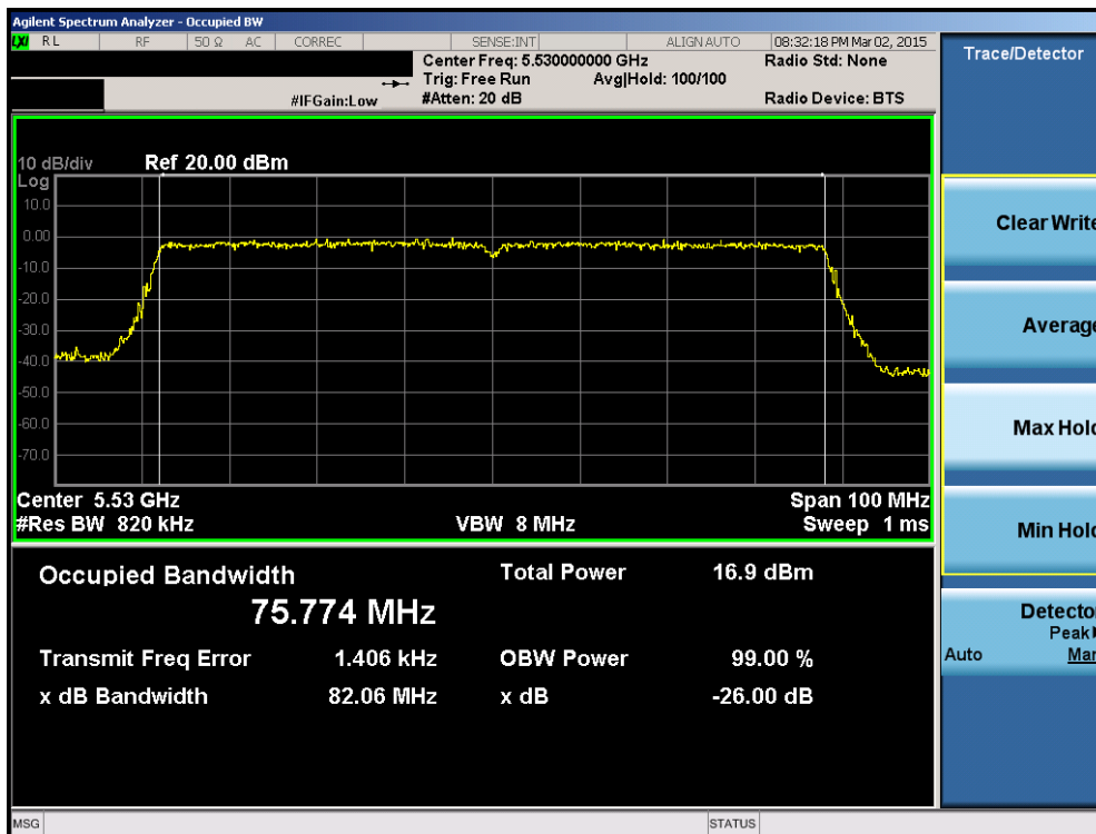
Plot 6-57. 26dB Bandwidth Plot (80MHz BW 802.11ac (UNII Band 2C) – Ch. 106)
