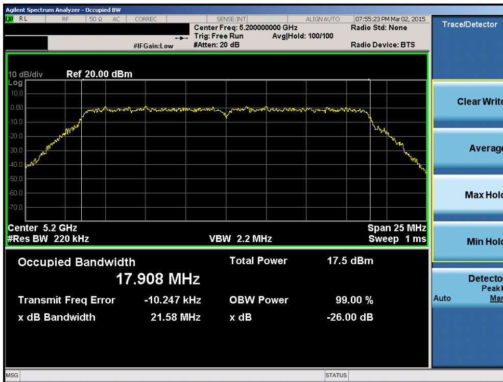
Plot 6-34. 26dB Bandwidth Plot (20MHz BW 802.11n (UNII Band 1) – Ch. 40)
