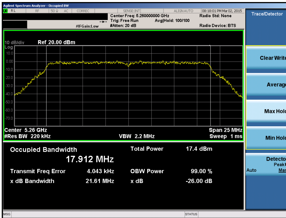
Plot 6-42. 26dB Bandwidth Plot (20MHz BW 802.11n (UNII Band 2A) – Ch. 52)
