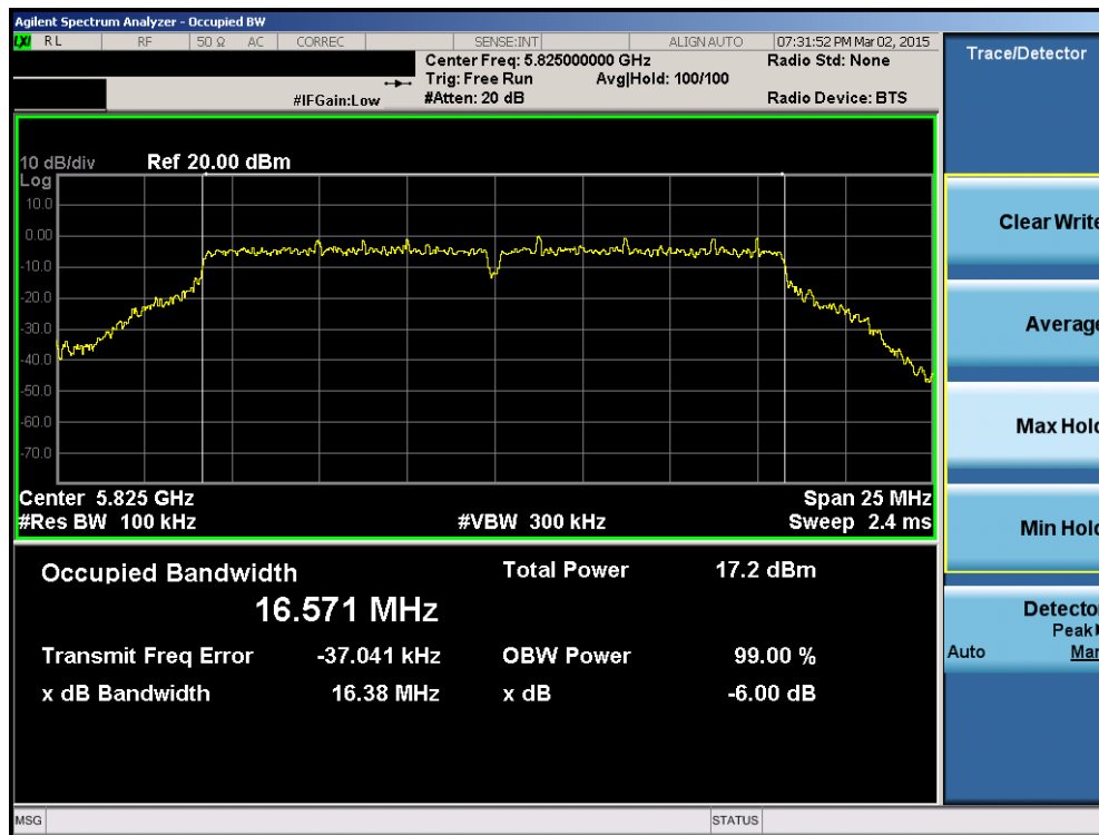
Plot 6-64. 6dB Bandwidth Plot (20MHz BW 802.11n (UNII Band 3) – Ch. 165)
