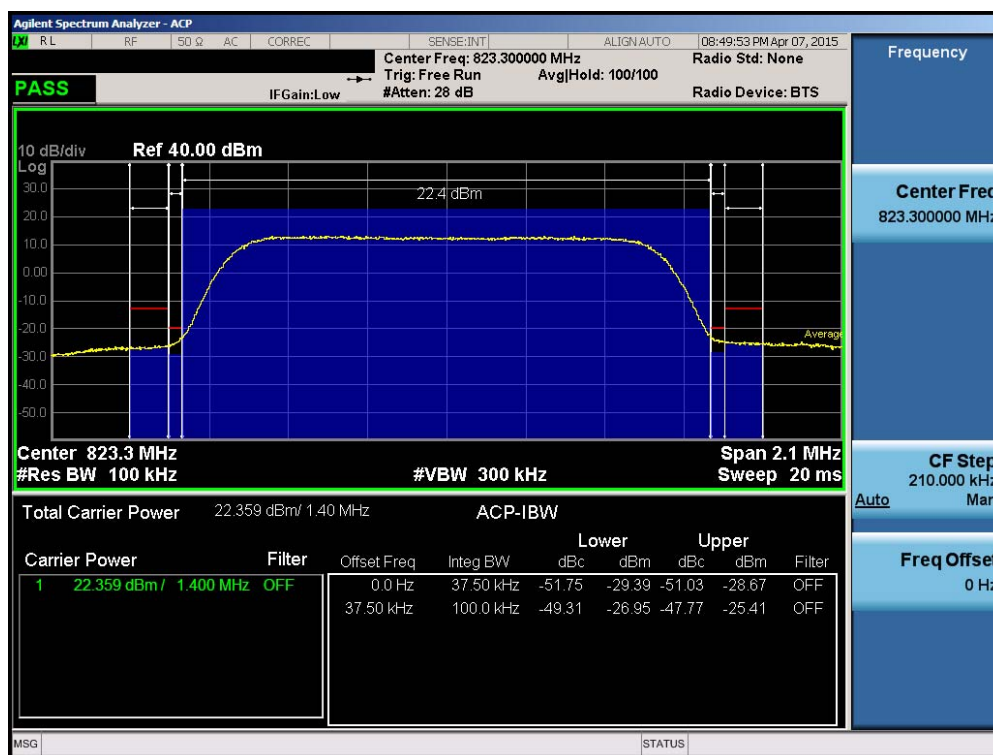
Plot 7-8. Channel Edge Plot (1.4MHz QPSK – RB Size 6 – High Channel)
