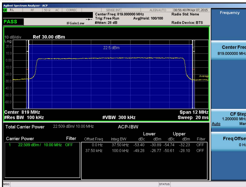
Plot 7-25. Channel Edge Plot (10MHz QPSK – RB Size 50)
