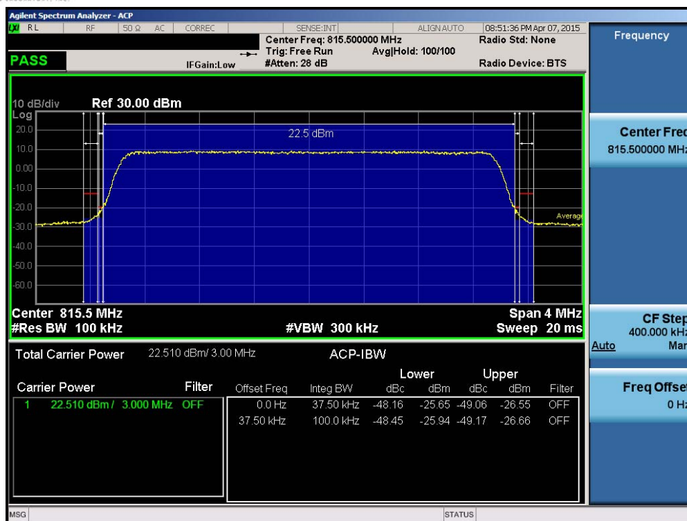
Plot 7-11. Channel Edge Plot (3MHz QPSK – RB Size 15– Low Channel)
