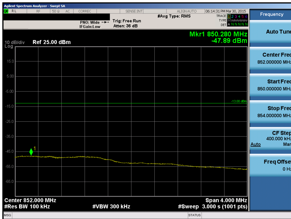
Plot 6-48. Upper Extended Band Edge Plot (Band 26 – 5.0MHz QPSK – RB Size 25)
