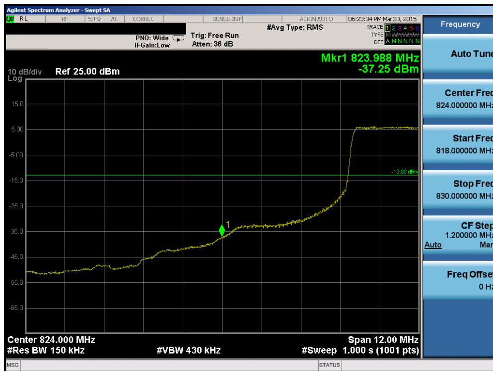
Plot 6-51. Lower Band Edge Plot (Band 26 – 15.0MHz QPSK – RB Size 75)
