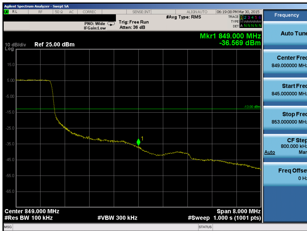
Plot 6-50. Upper Band Edge Plot (Band 26 – 10.0MHz QPSK – RB Size 50)
