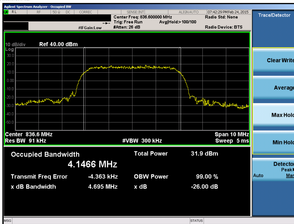
Plot 6-5. Occupied Bandwidth Plot (Cellular WCDMA Mode – Ch. 4183)
