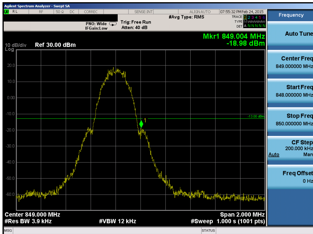
Plot 6-34. Band Edge Plot (Cellular GSM Mode – Ch. 251)
