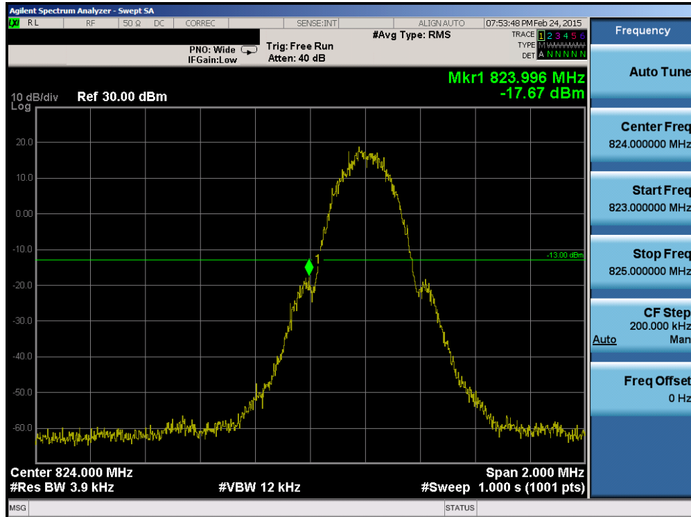
Plot 6-33. Band Edge Plot (Cellular GSM Mode – Ch. 128)
