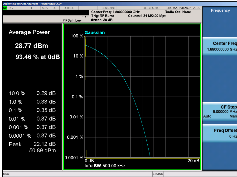
Plot 6-41. Peak-Average Ratio Plot (PCS GSM Mode – Ch. 661)
