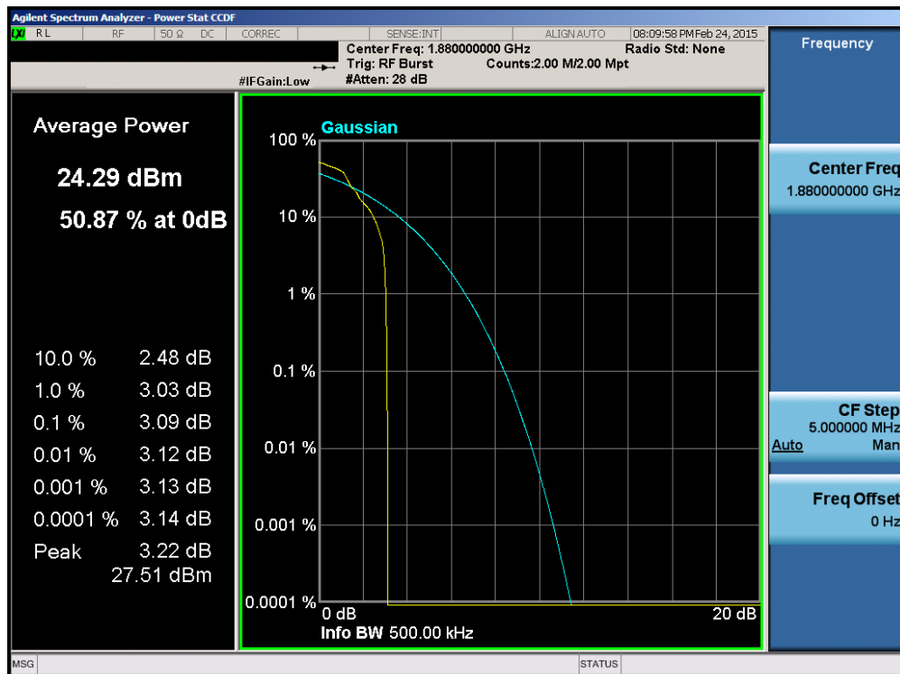
Plot 6-42. Peak-Average Ratio Plot (EDGE1900 Mode – Ch. 661)
