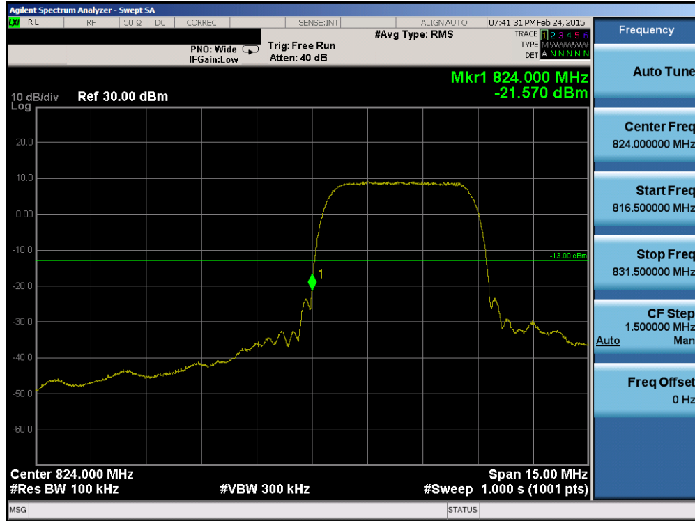
Plot 6-39. Band Edge Plot (Cellular WCDMA Mode – Ch. 4132)
