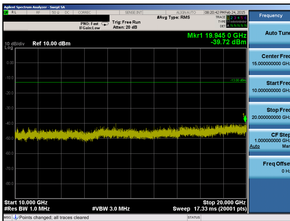
Plot 6-23. Conducted Spurious Plot (PCS GSM Mode – Ch. 810)
