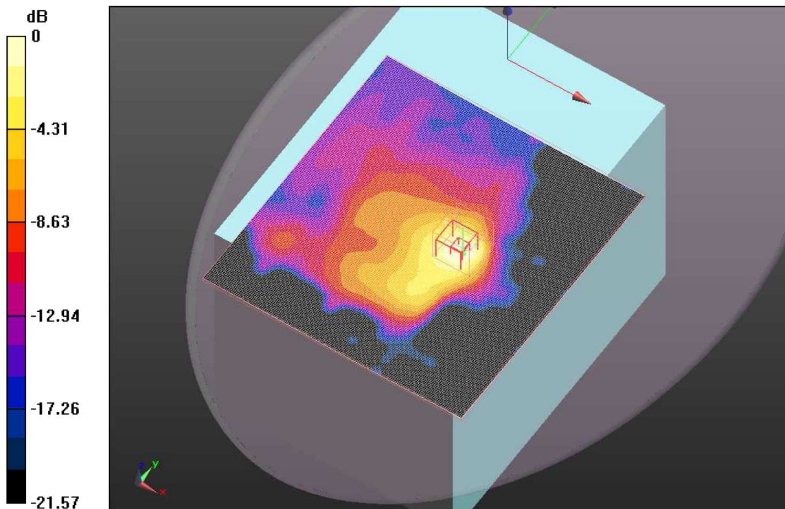
0 dB = 0.270mW/g
