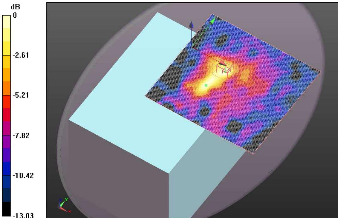
0 dB = 0.070mW/g
