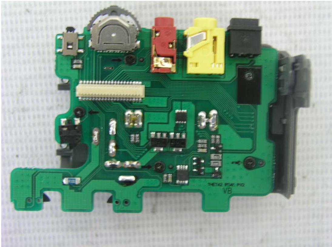
SUB board
