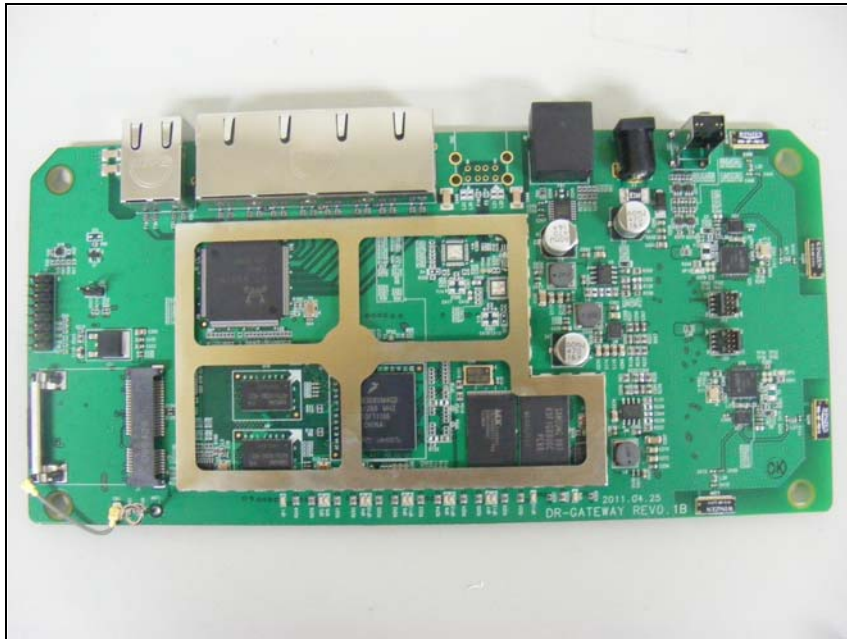
PCB top view (Main Board)
