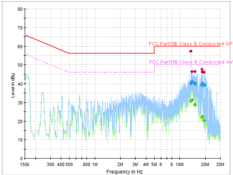
Plot 7-5. Line-Conducted Test Plot (L1)
