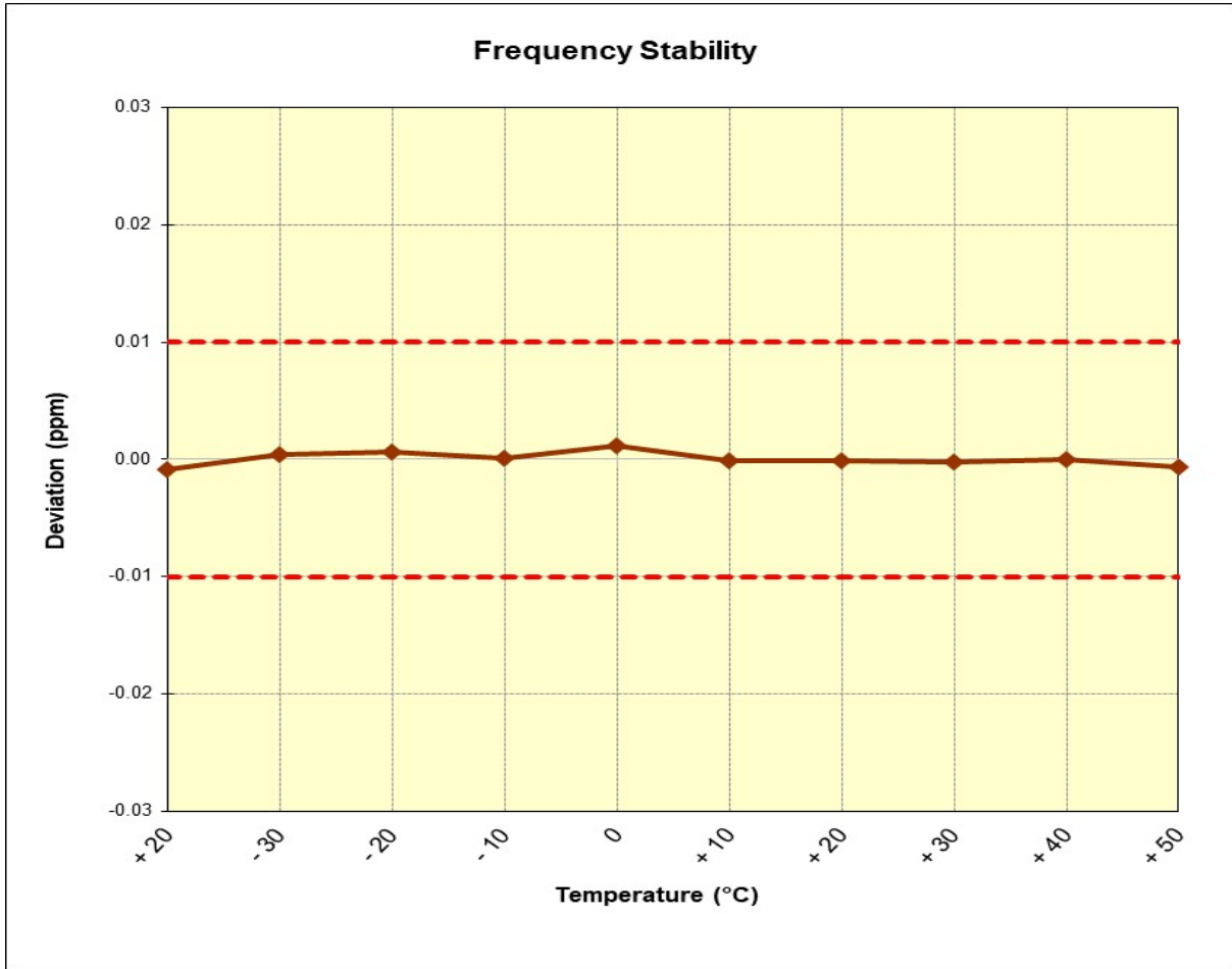
Figure 7-3. Frequency Stability Plot
