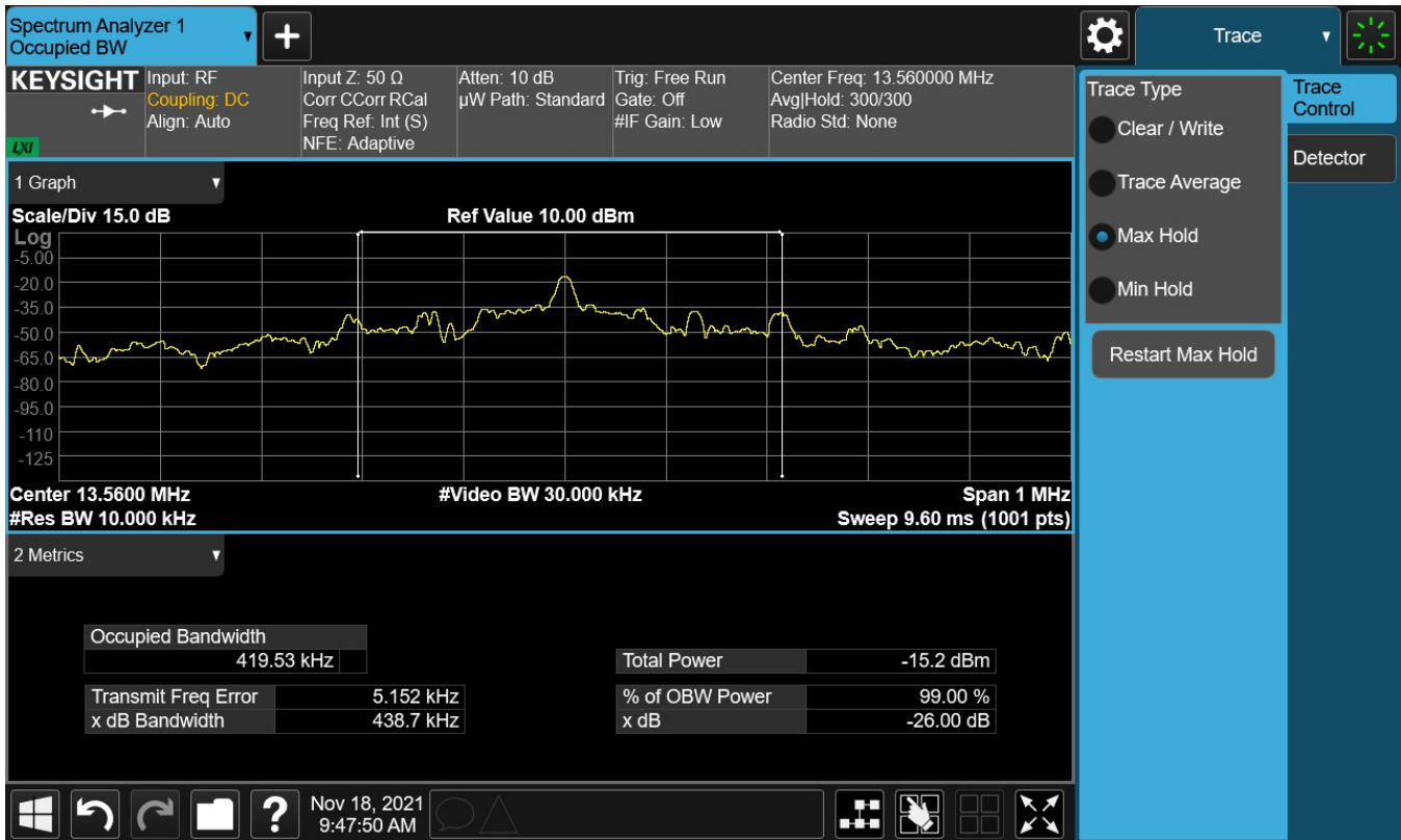
Figure 7-2. Occupied Bandwidth Plot
