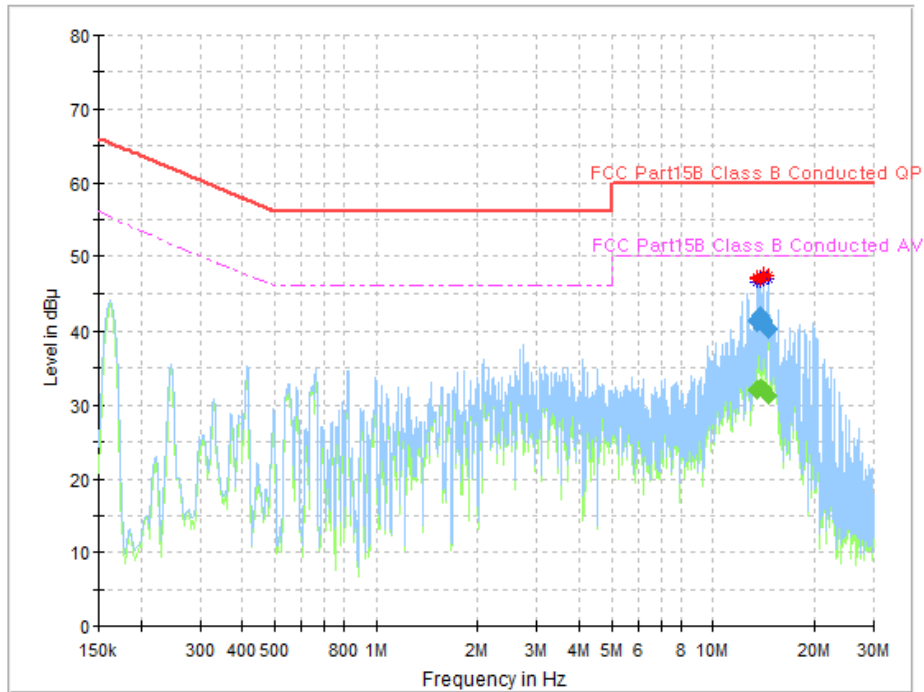
Plot 7-6. Line-Conducted Test Plot (N)
