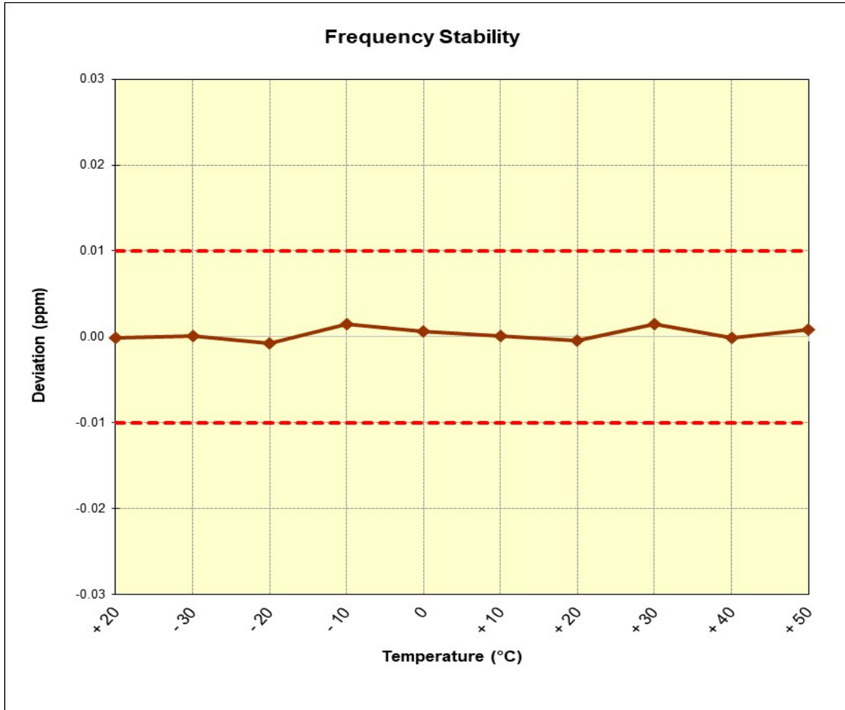
Figure 7-3. Frequency Stability Plot
