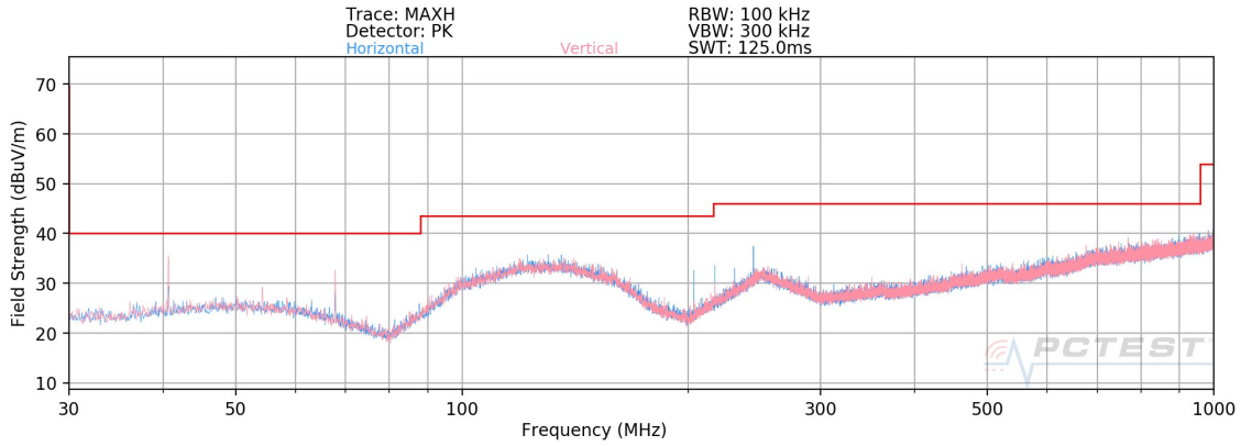
Plot 7-4. Radiated Spurious Plot 30MHz – 1GHz
