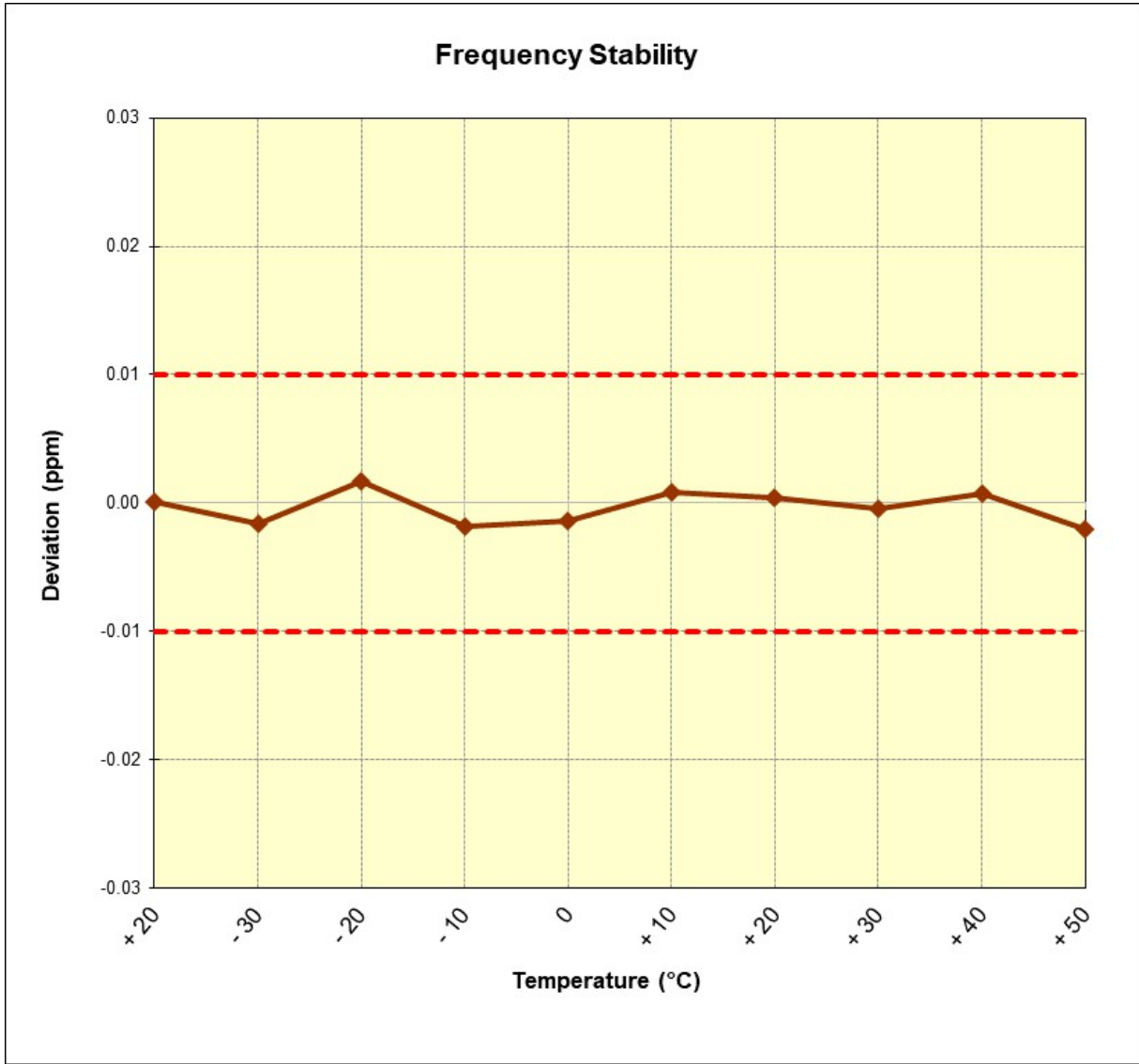
Figure 7-3. Frequency Stability Plot
