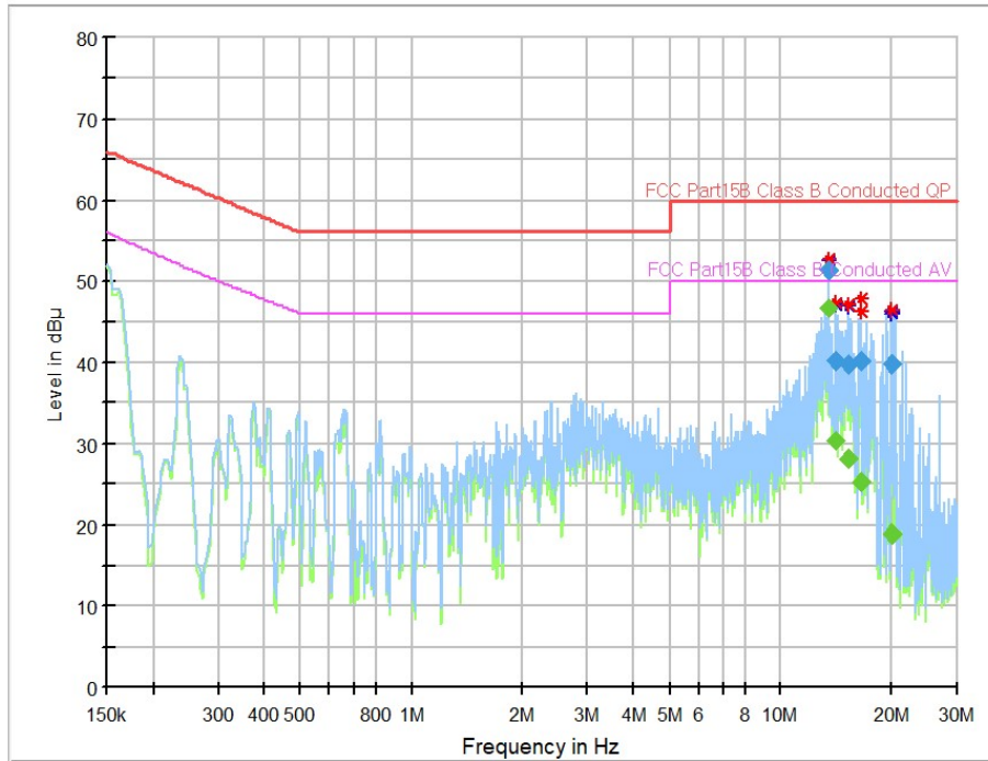
Plot 7-5. Line-Conducted Plot (L1)
