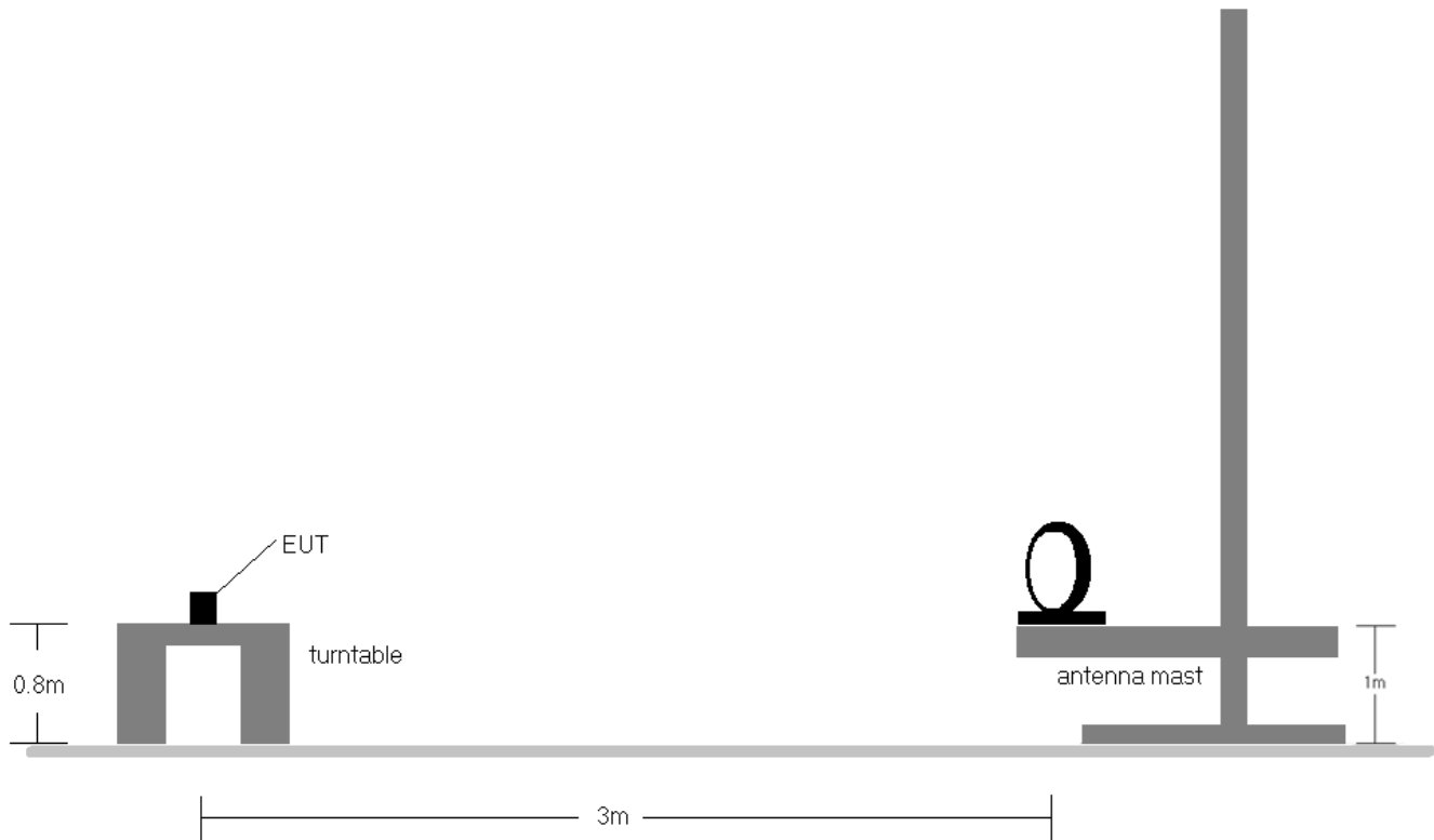
Figure 7-4. Radiated Test Setup
