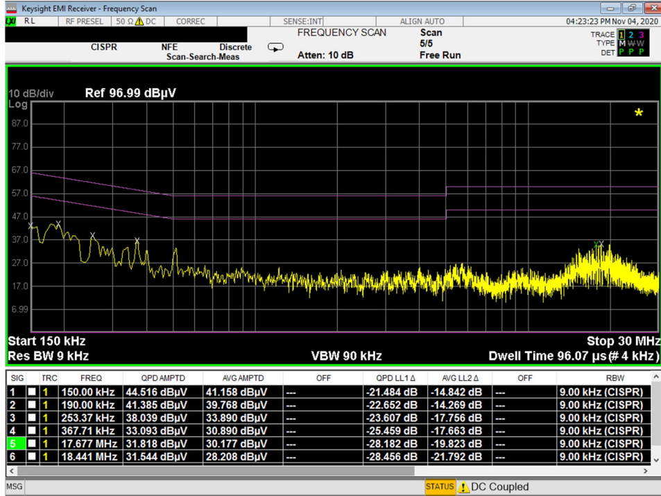
Plot 7-4. Line-Conducted Test Plot (L1) with Antenna Terminated in 50Ω
