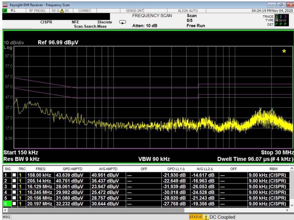
Plot 7-5. Line-Conducted Test Plot (N) with Antenna Terminated in 50Ω
