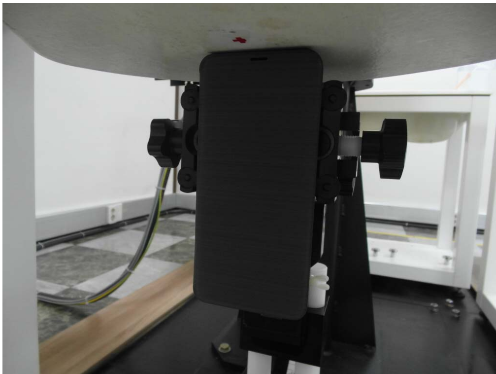
Cell Phone + LED Cover Top Phablet
