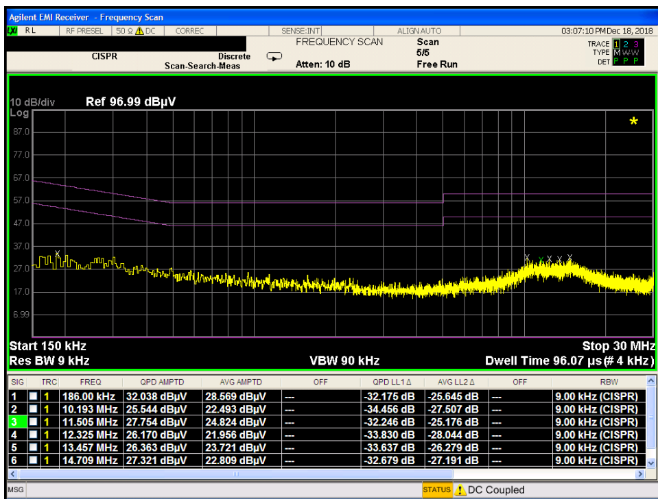
Plot 7-7. Line-Conducted Test Plot (L1) – with Antenna Terminated in 50Ω
