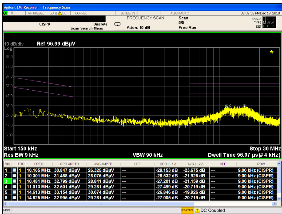
Plot 7-8. Line-Conducted Test Plot (N) – with Antenna Terminated in 50Ω
