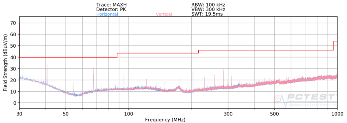
Plot 7-4. Radiated Spurious Plot 30MHz – 1GHz (Pol. H/V)
