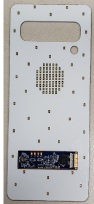
ANT-LED Module(Back)
