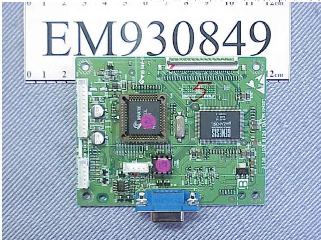
Figure 13 Internal View (Main Board/Component Side)
