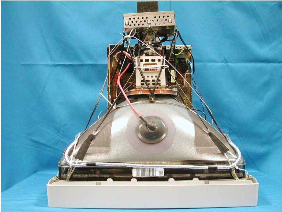
Top View w/o Back cover (SAMSUNG)
