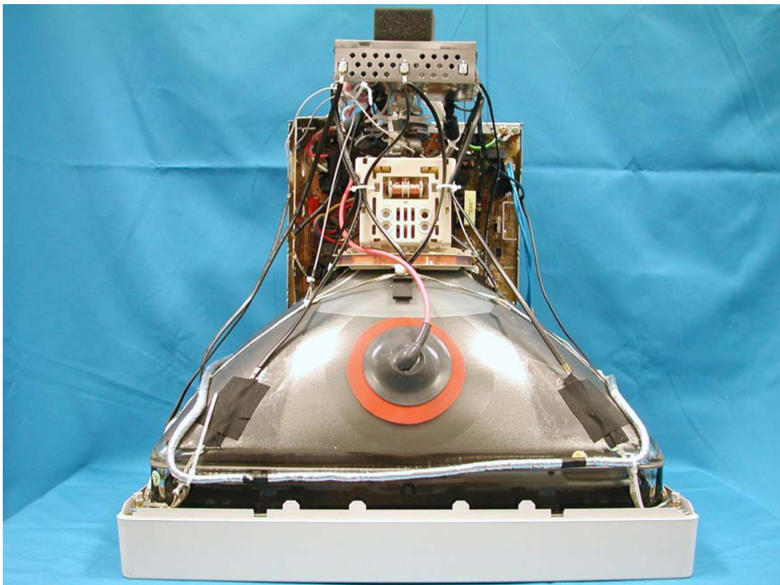
Top View w/o Back cover (CHUNGHWA)
