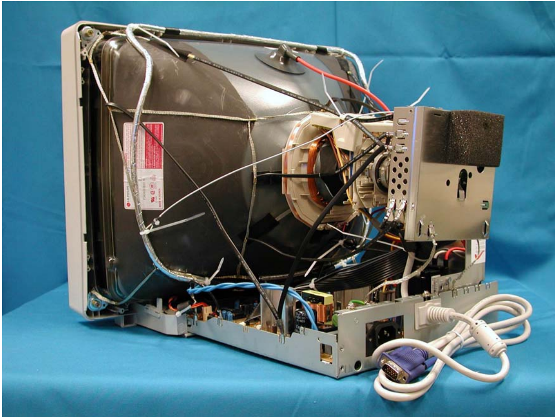
Left View w/o Back Cover (LG.PHILIPS)
