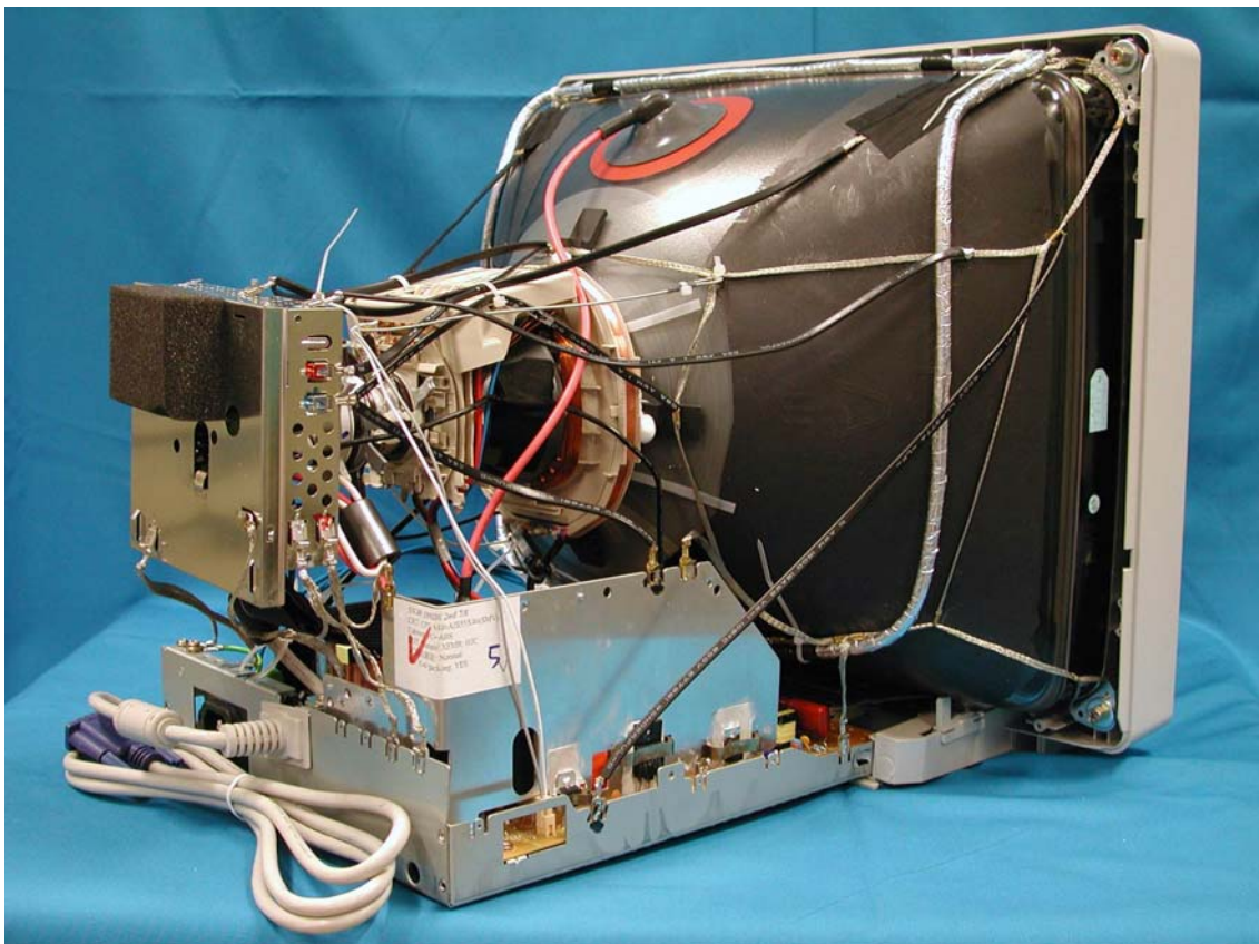
Right View w/o Back cover (CHUNGHWA)
