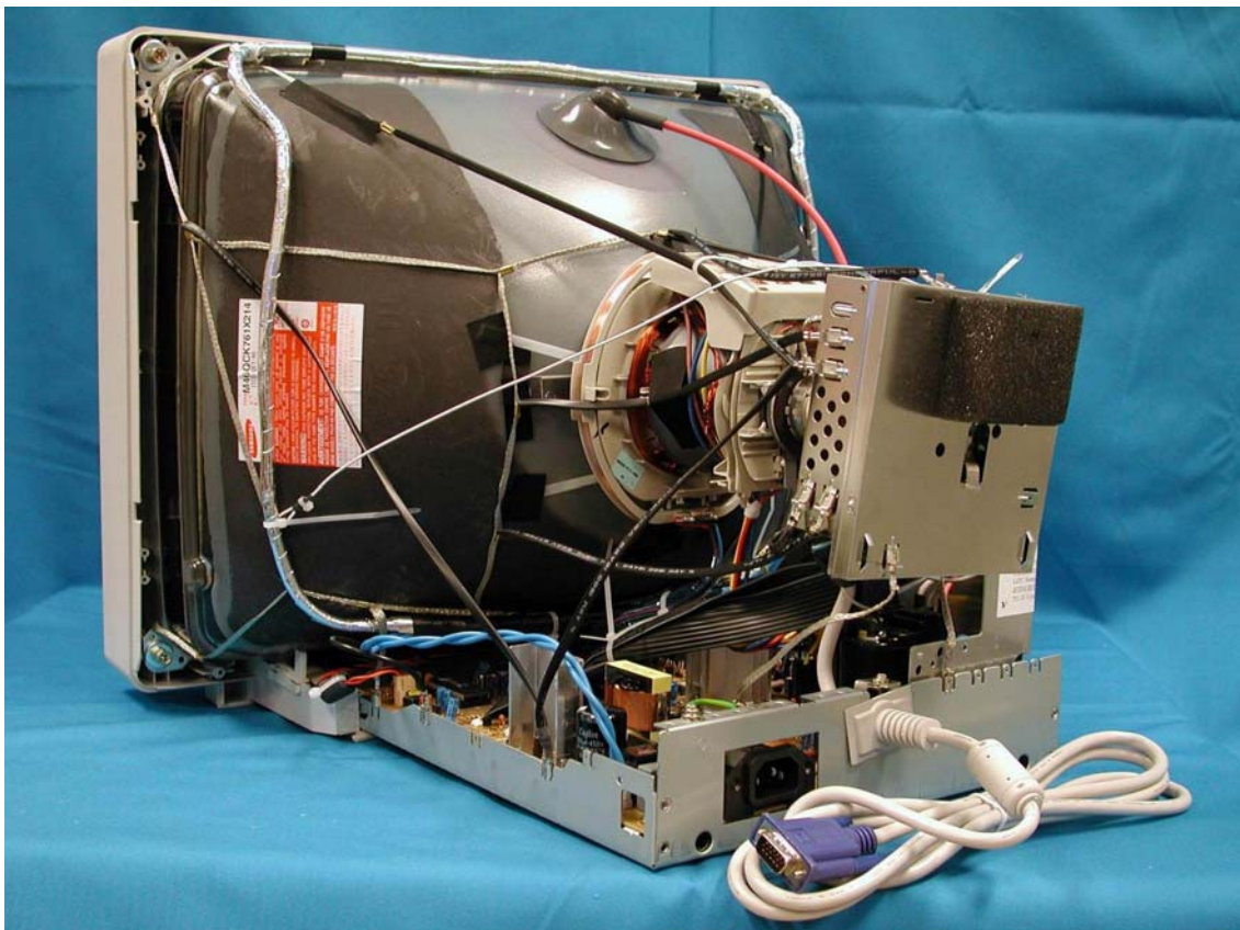
Left View w/o Back cover (SAMSUNG)
