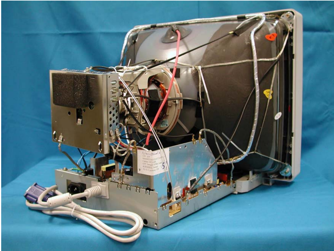
Right View w/o Back cover (SAMSUNG)
