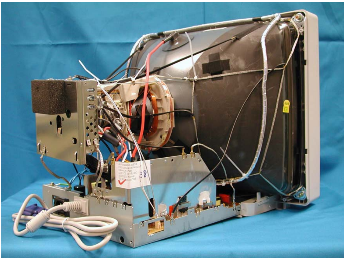
Right View w/o Back Cover (LG.PHILIPS)
