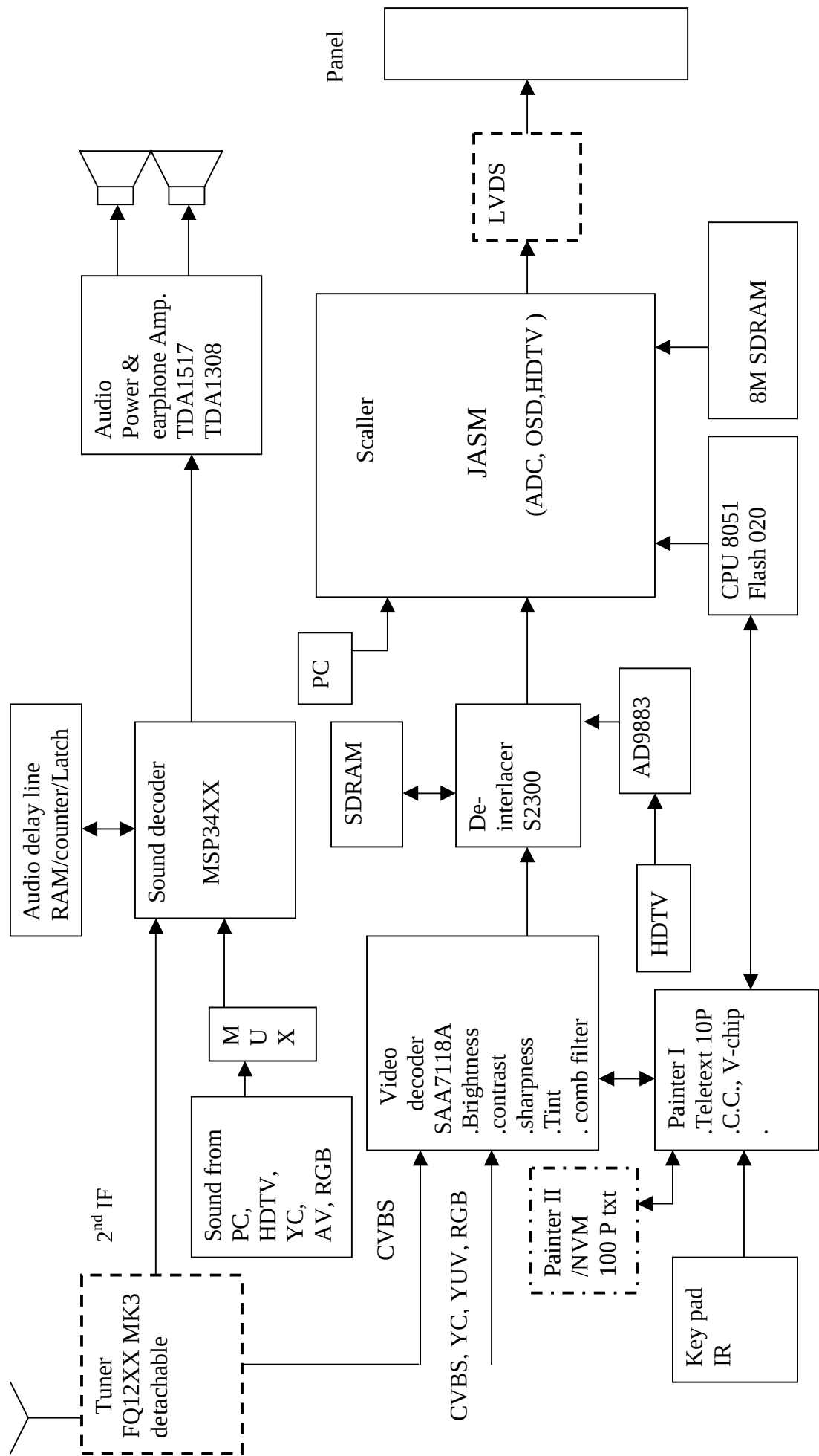
150MT2 LCD TV-Monitor Function Block
