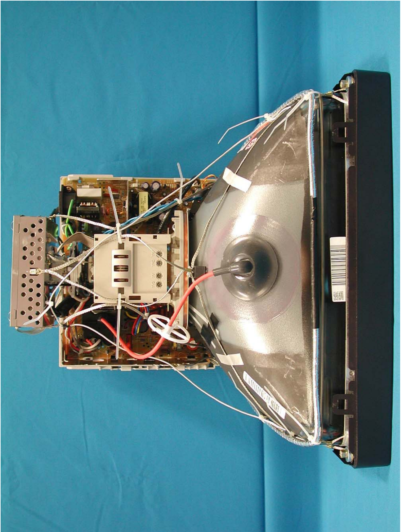
Top View Without Back Cover (SAMSUNG)
