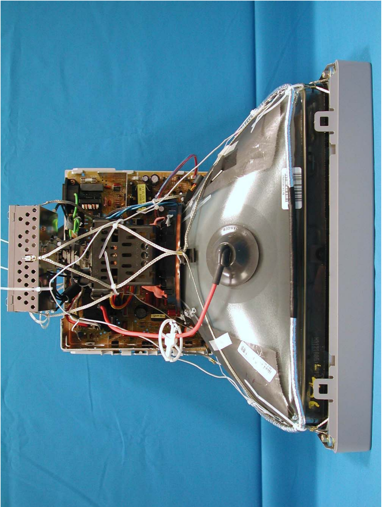
Top View Without Back Cover (LG.PHILIPS)
