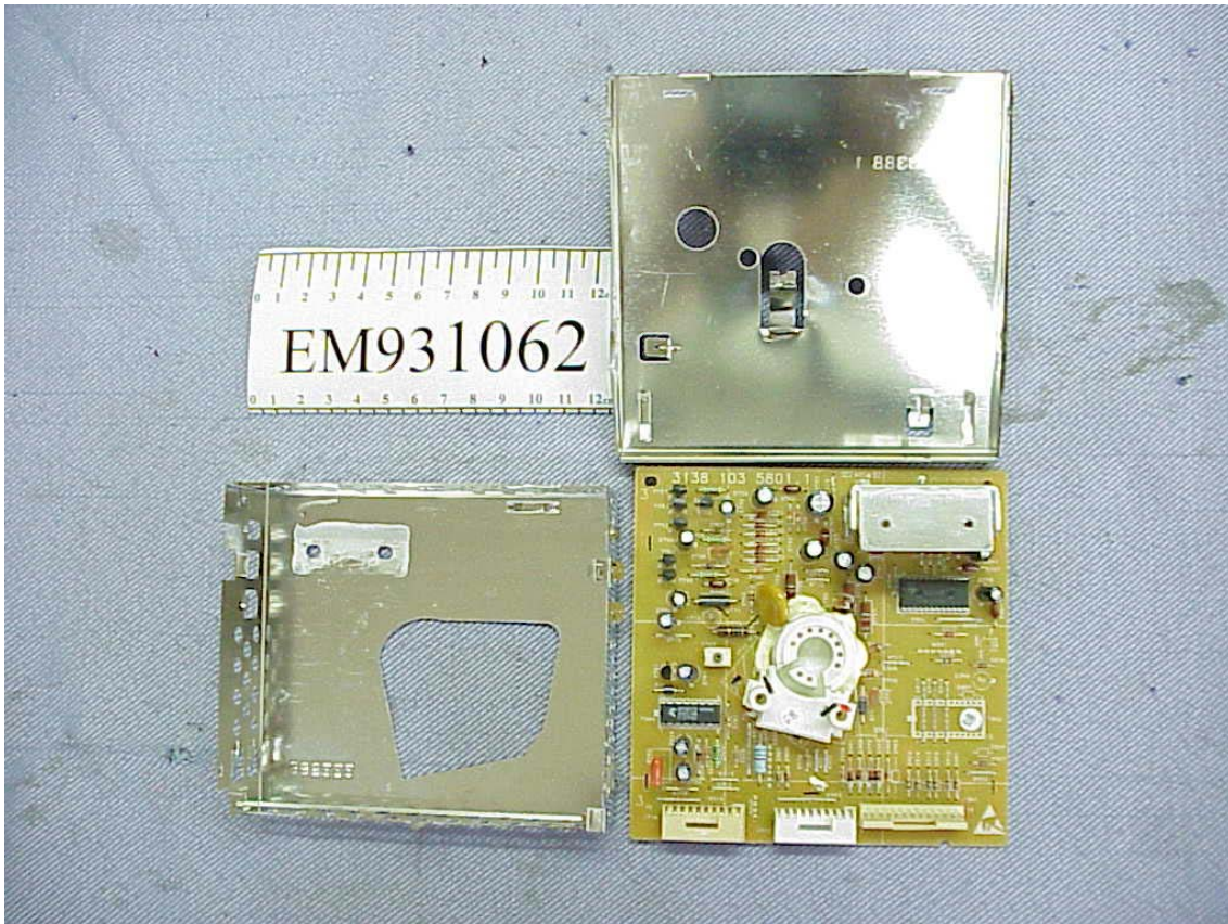
PCB Layout with shielding
