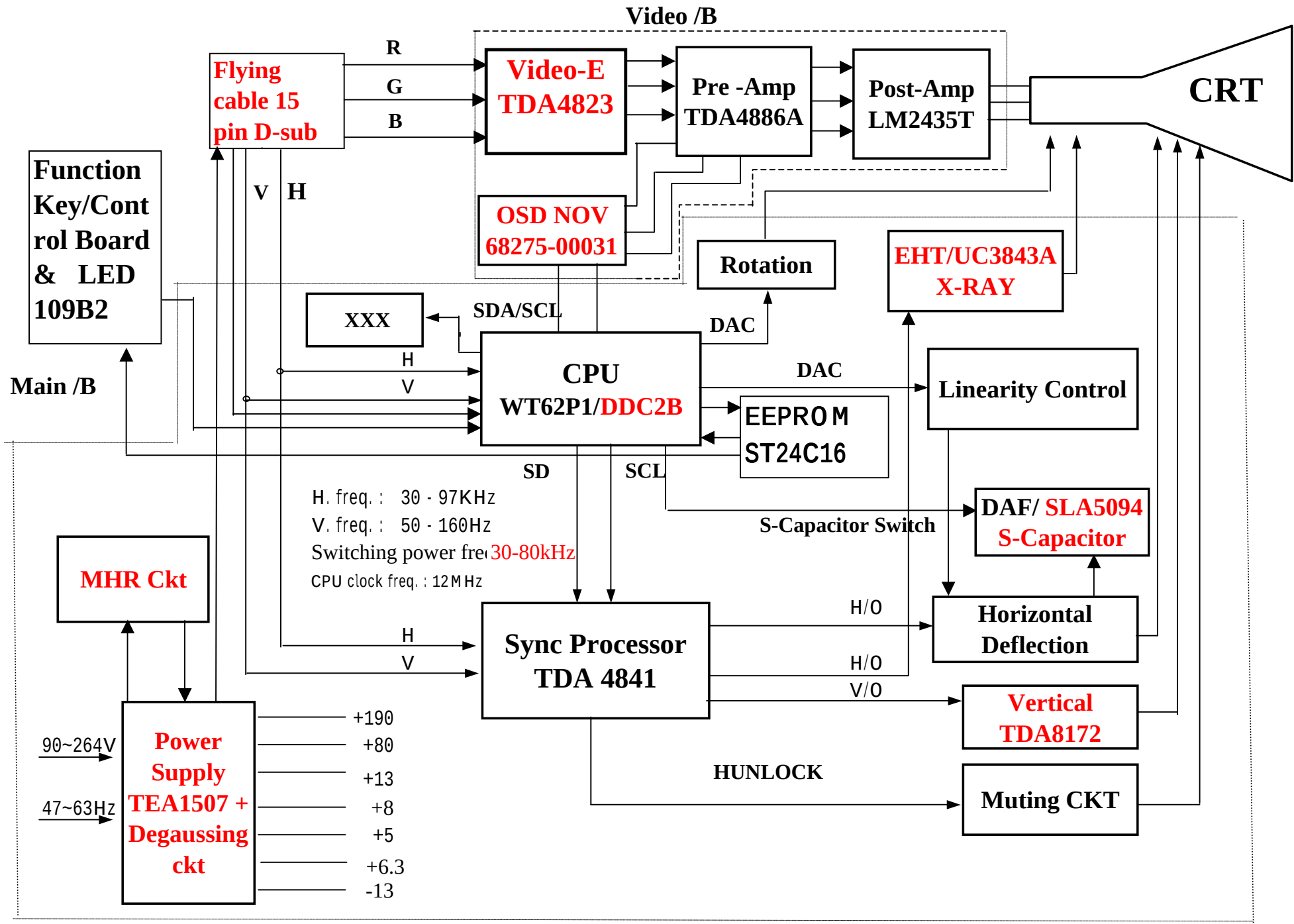
Exhibit 5: Block Diagram
