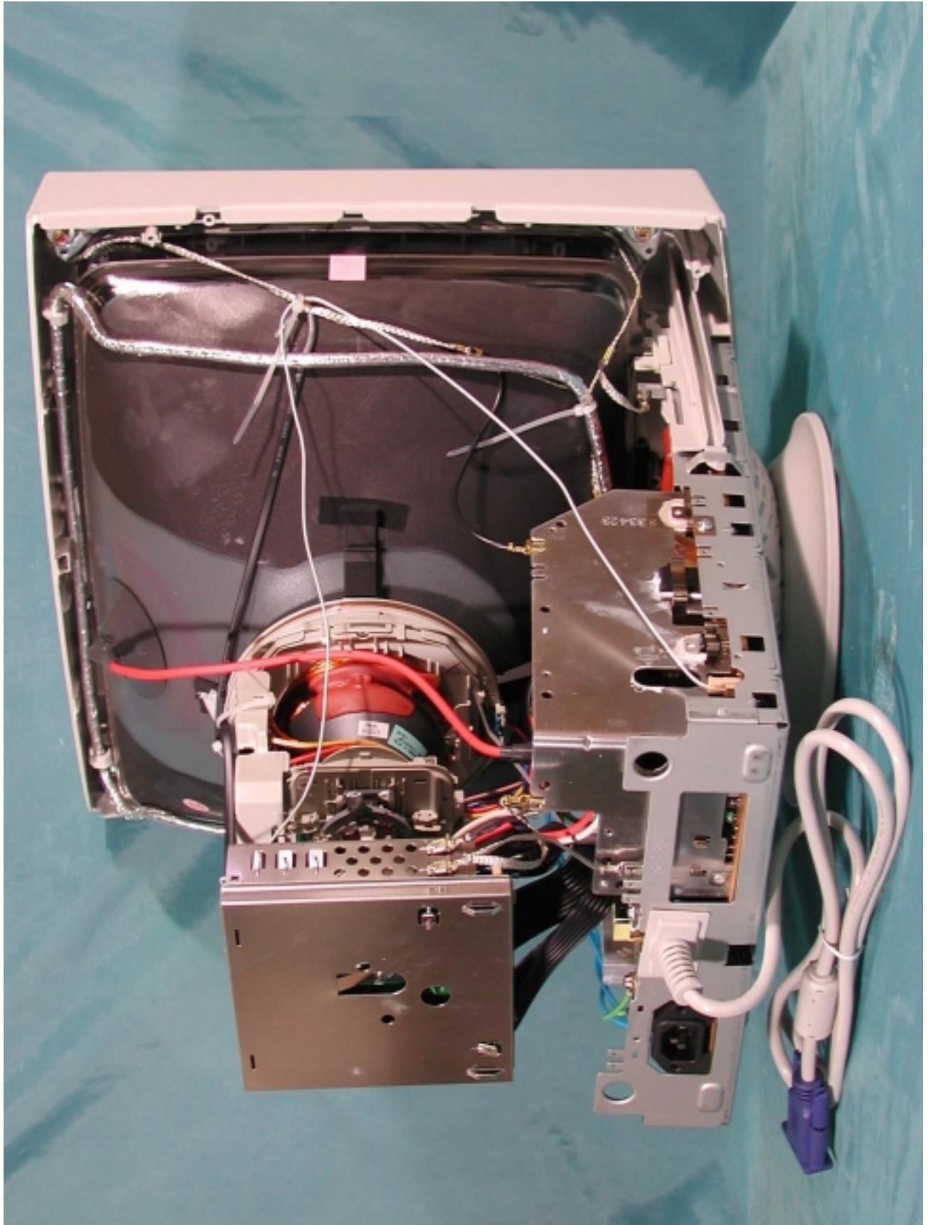
Side View Without Back Cover
