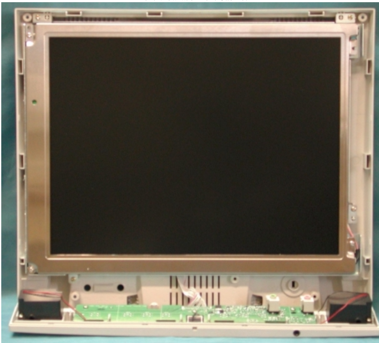
Front View w/o Front Cabinet
