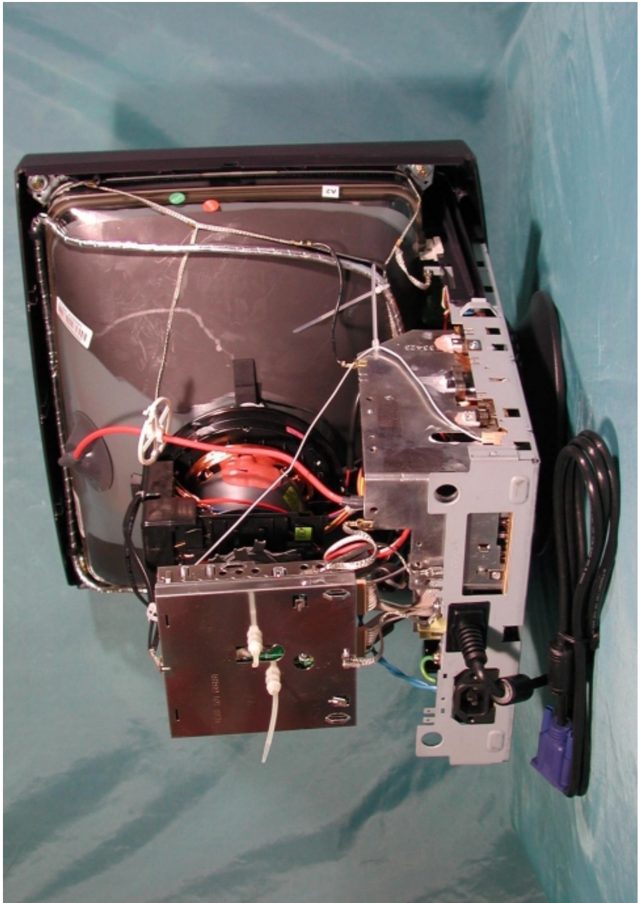
Side View Without Back Cover
