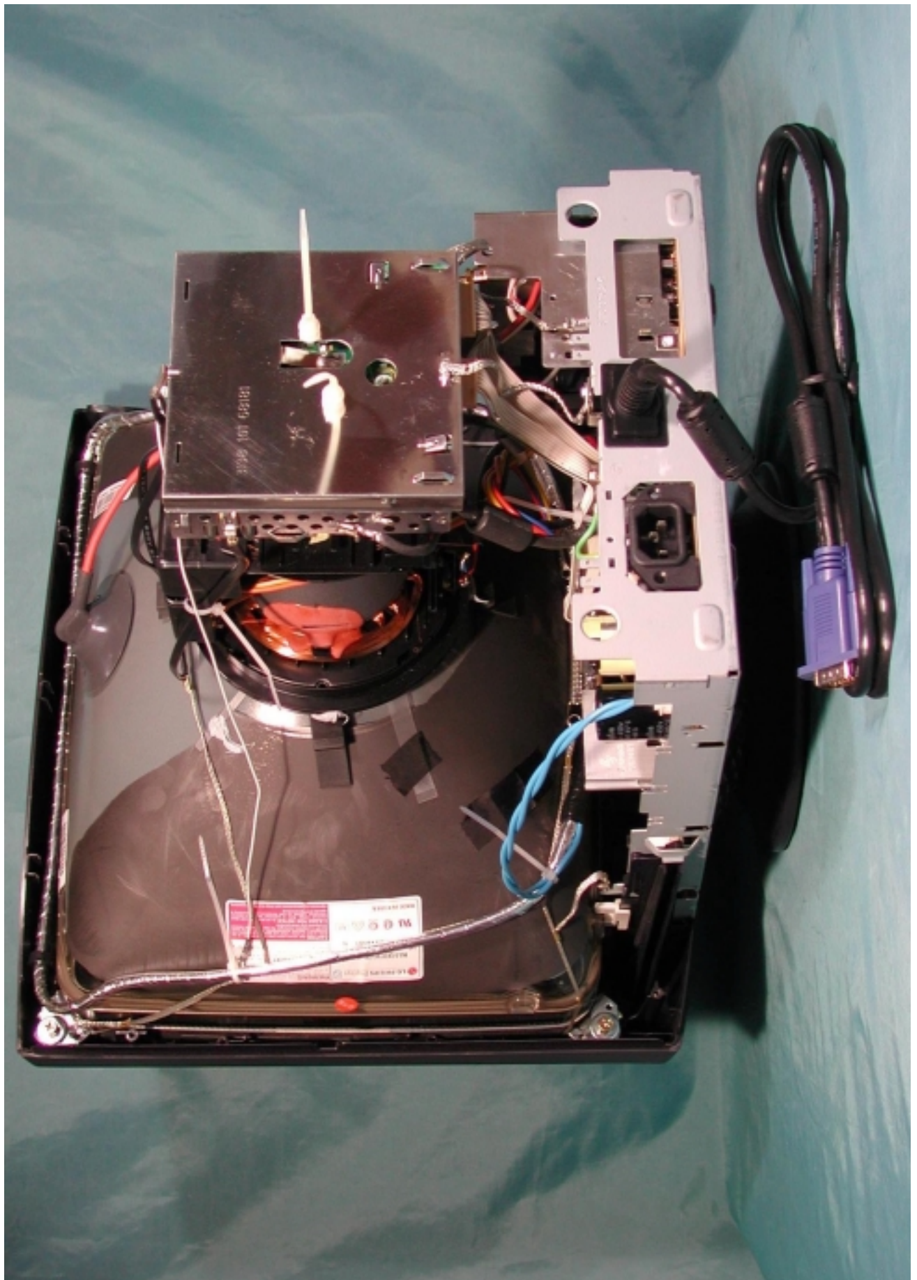
Side View Without Back Cover
